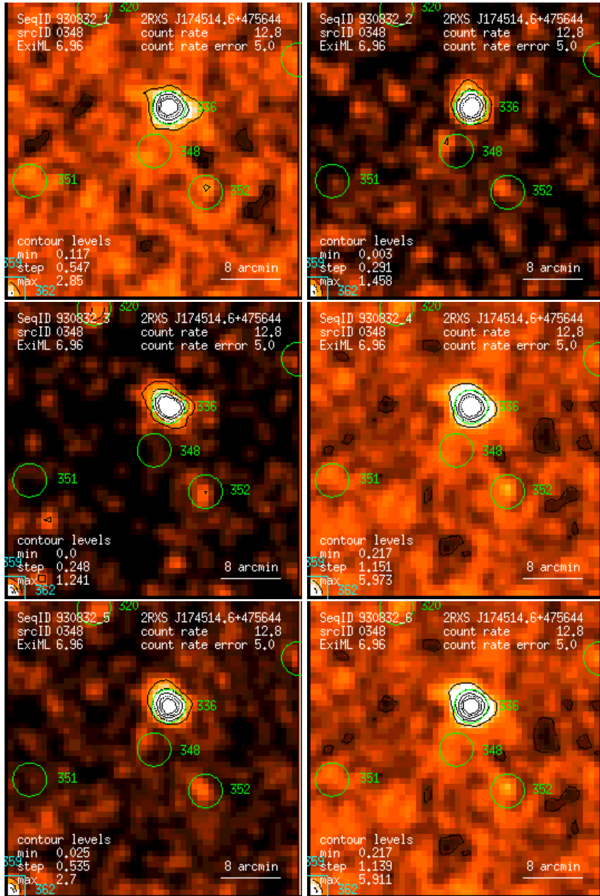
Figure 348: RASS 930832: detection 0348: band rate images, Gaussian filter: (1) PSPC channels 11 – 41, (2) 52 – 90, (3) 91 – 201, (4) 11 – 235, (5) 52 – 201, (6) 11 – 201. Broad band rates in counts/ks. Band rate contour levels in counts/ks/arcmin 2 .
