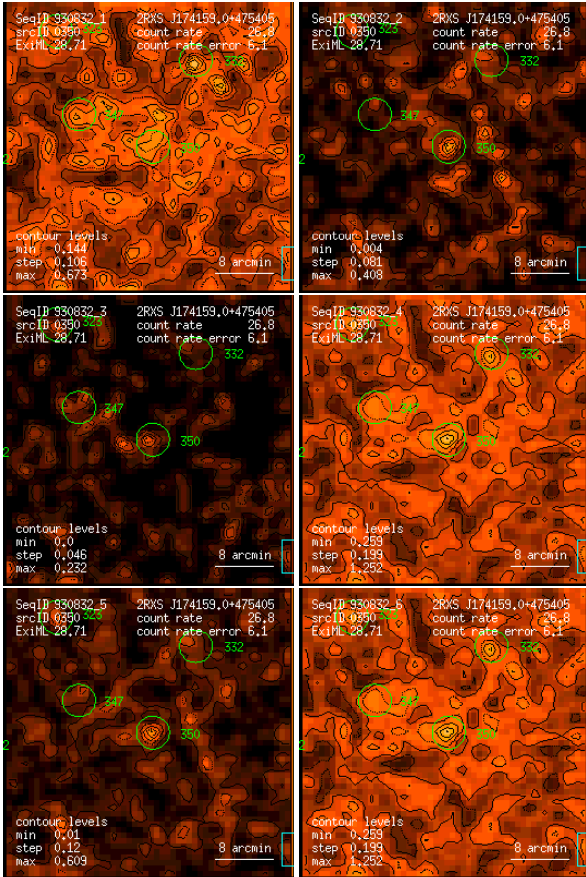
Figure 350: RASS 930832: detection 0350: band rate images, Gaussian filter: (1) PSPC channels 11 – 41, (2) 52 – 90, (3) 91 – 201, (4) 11 – 235, (5) 52 – 201, (6) 11 – 201. Broad band rates in counts/ks. Band rate contour levels in counts/ks/arcmin 2 .
