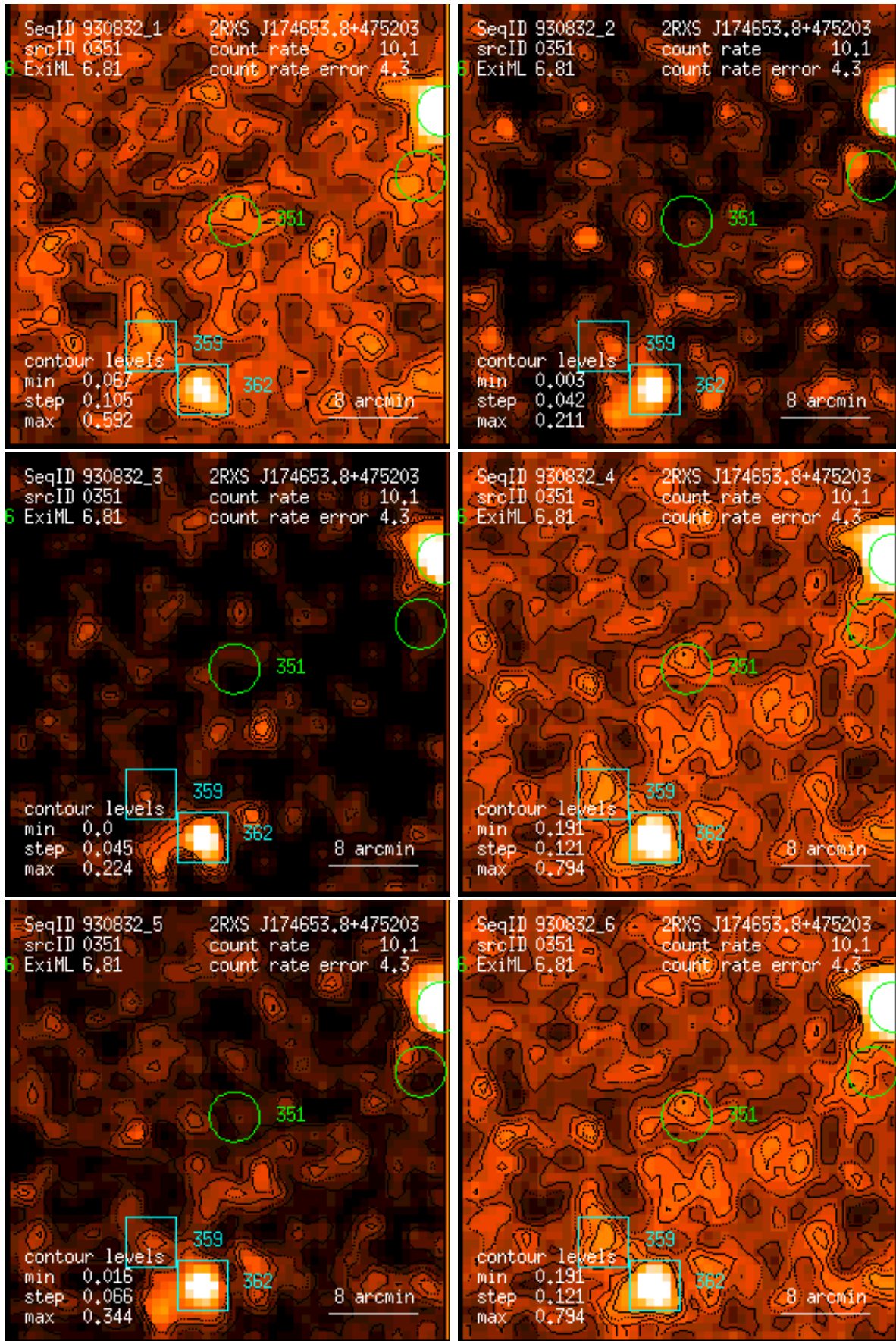
Figure 351: RASS 930832: detection 0351: band rate images, Gaussian filter: (1) PSPC channels 11 – 41, (2) 52 – 90, (3) 91 – 201, (4) 11 – 235, (5) 52 – 201, (6) 11 – 201. Broad band rates in counts/ks. Band rate contour levels in counts/ks/arcmin 2 .
