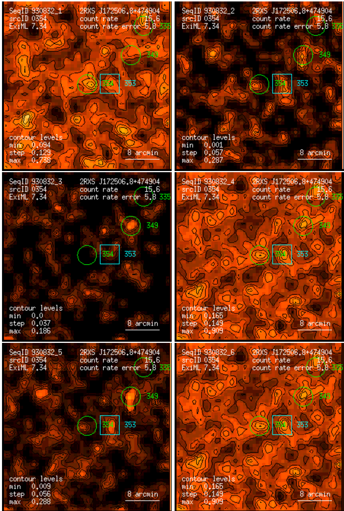
Figure 354: RASS 930832: detection 0354: band rate images, Gaussian filter: (1) PSPC channels 11 – 41, (2) 52 – 90, (3) 91 – 201, (4) 11 – 235, (5) 52 – 201, (6) 11 – 201. Broad band rates in counts/ks. Band rate contour levels in counts/ks/arcmin 2 .
