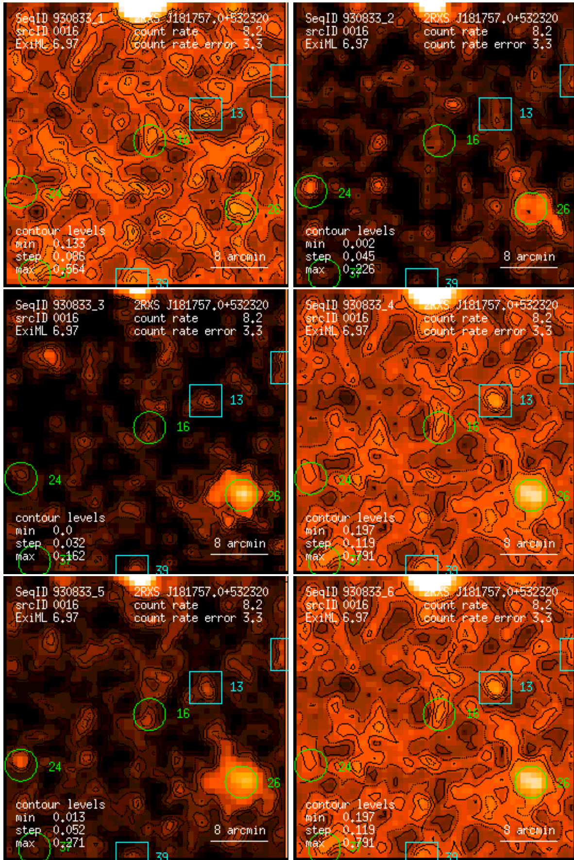
Figure 16: RASS 930833: detection 0016: band rate images, Gaussian filter: (1) PSPC channels 11 – 41, (2) 52 – 90, (3) 91 – 201, (4) 11 – 235, (5) 52 – 201, (6) 11 – 201. Broad band rates in counts/ks. Band rate contour levels in counts/ks/arcmin 2 .
