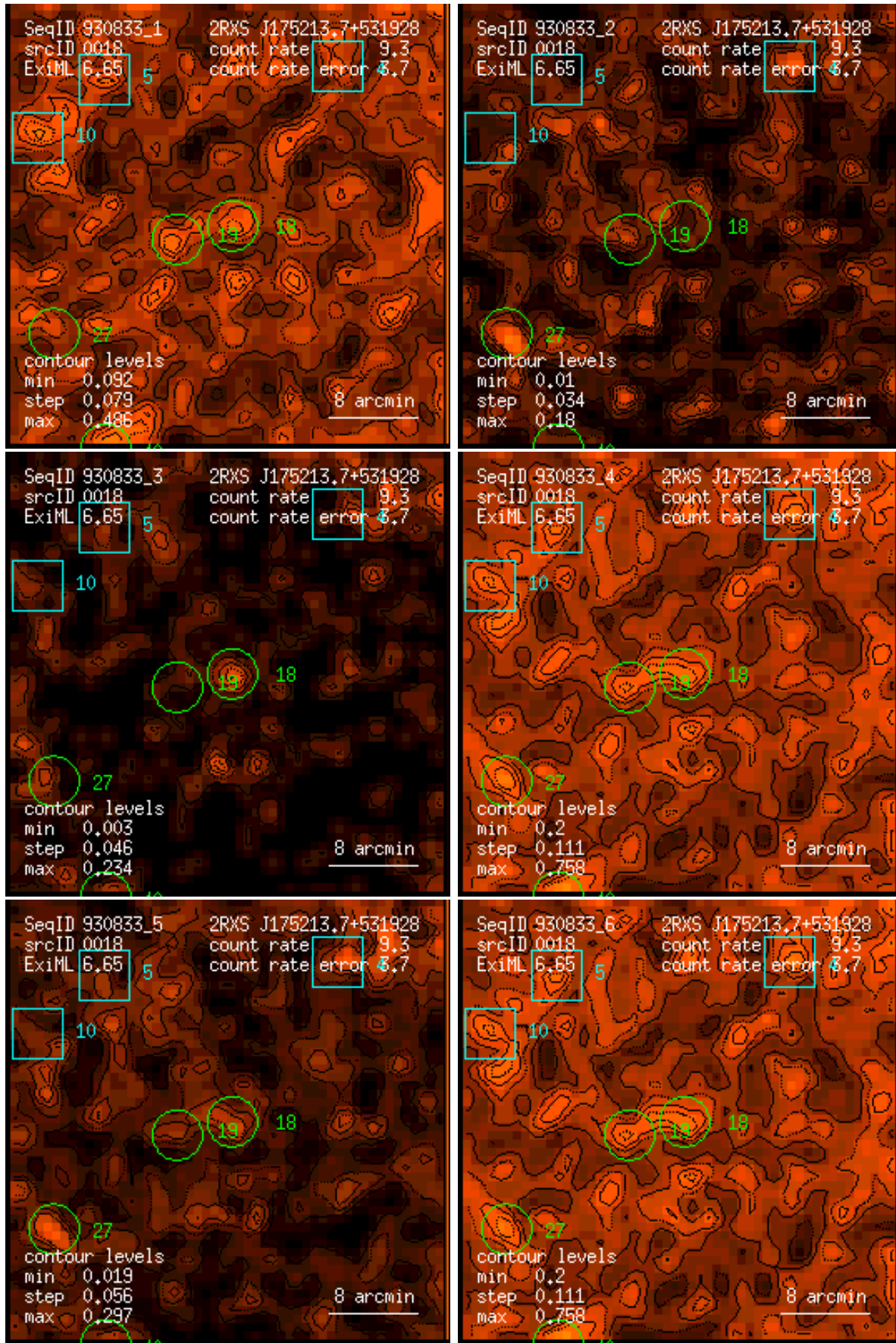
Figure 18: RASS 930833: detection 0018: band rate images, Gaussian filter: (1) PSPC channels 11 – 41, (2) 52 – 90, (3) 91 – 201, (4) 11 – 235, (5) 52 – 201, (6) 11 – 201. Broad band rates in counts/ks. Band rate contour levels in counts/ks/arcmin 2 .
