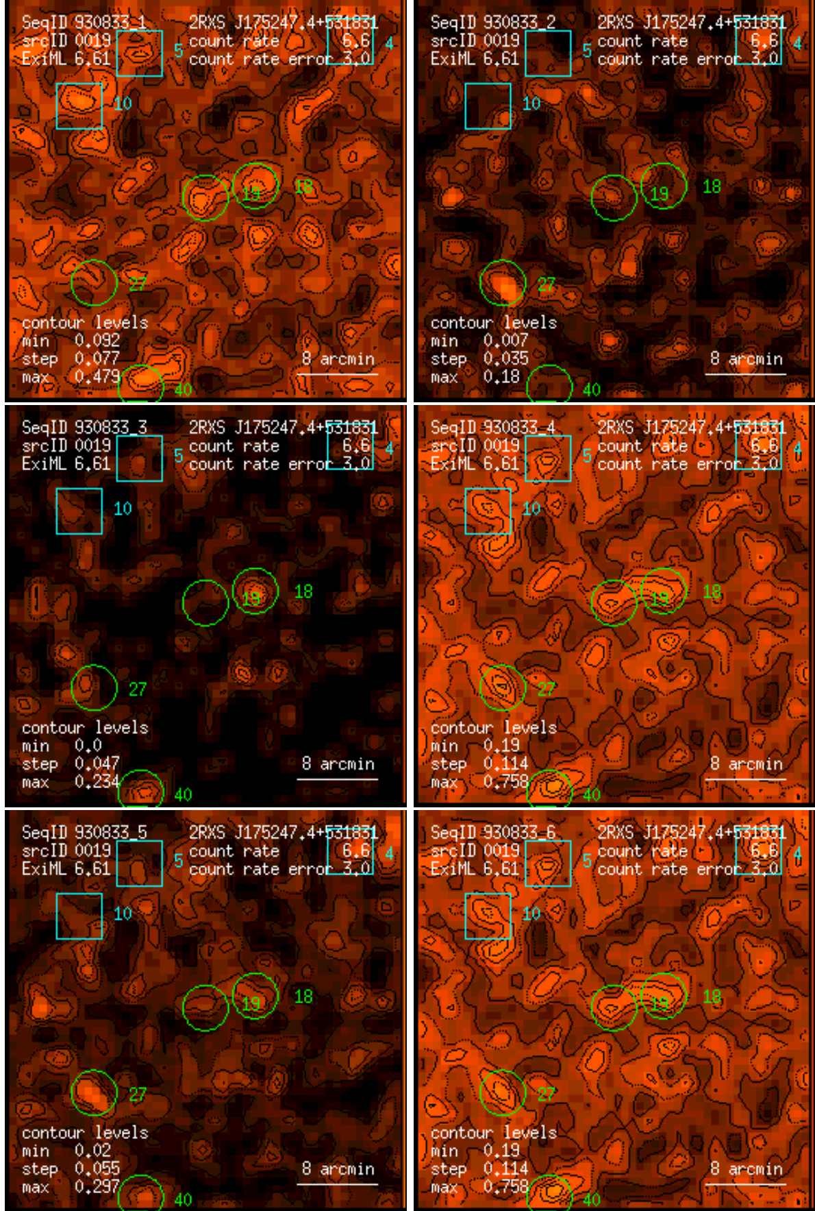
Figure 19: RASS 930833: detection 0019: band rate images, Gaussian filter: (1) PSPC channels 11 – 41, (2) 52 – 90, (3) 91 – 201, (4) 11 – 235, (5) 52 – 201, (6) 11 – 201. Broad band rates in counts/ks. Band rate contour levels in counts/ks/arcmin 2 .
