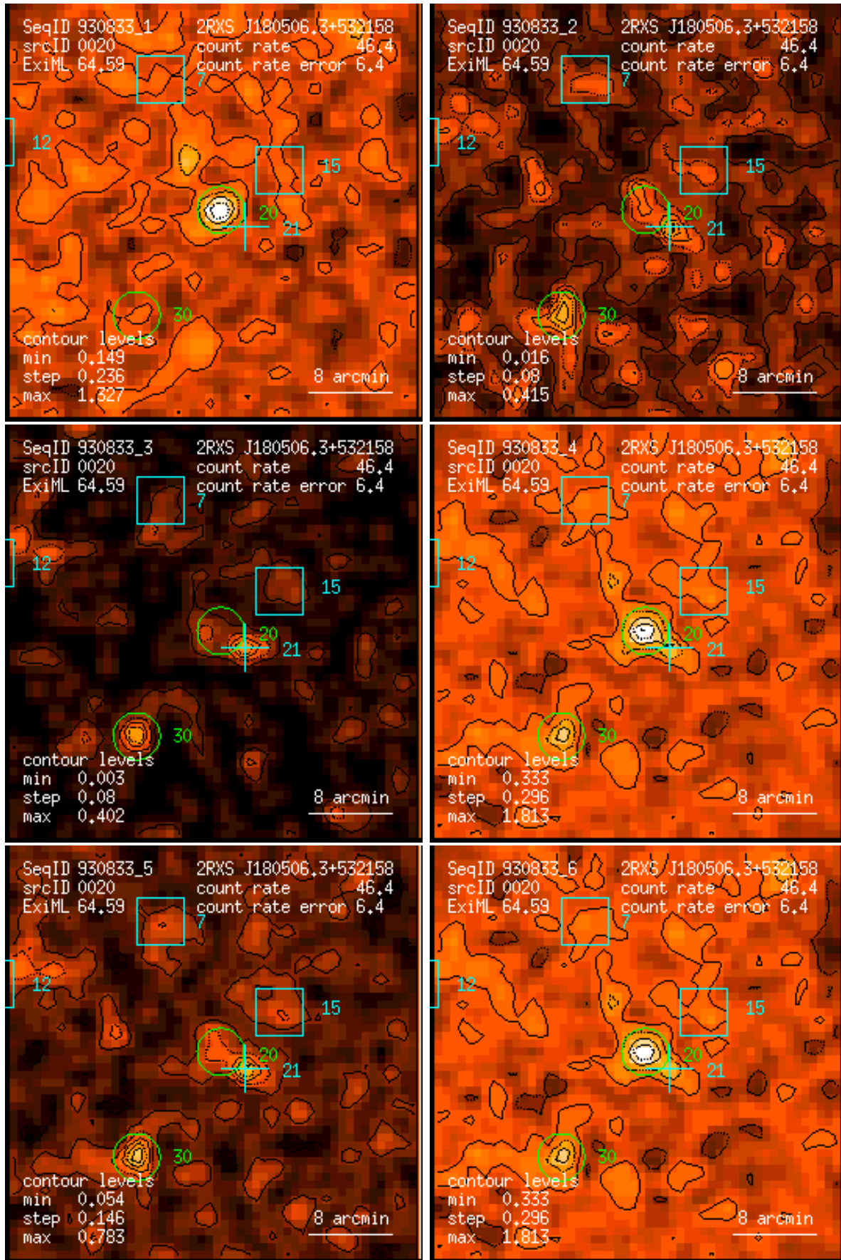
Figure 20: RASS 930833: detection 0020: band rate images, Gaussian filter: (1) PSPC channels 11 – 41, (2) 52 – 90, (3) 91 – 201, (4) 11 – 235, (5) 52 – 201, (6) 11 – 201. Broad band rates in counts/ks. Band rate contour levels in counts/ks/arcmin 2 .
