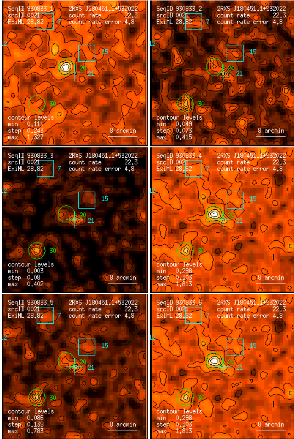
Figure 21: RASS 930833: detection 0021: band rate images, Gaussian filter: (1) PSPC channels 11 – 41, (2) 52 – 90, (3) 91 – 201, (4) 11 – 235, (5) 52 – 201, (6) 11 – 201. Broad band rates in counts/ks. Band rate contour levels in counts/ks/arcmin 2 .
