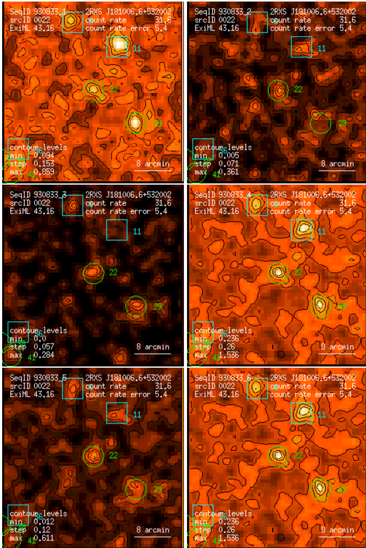
Figure 22: RASS 930833: detection 0022: band rate images, Gaussian filter: (1) PSPC channels 11 – 41, (2) 52 – 90, (3) 91 – 201, (4) 11 – 235, (5) 52 – 201, (6) 11 – 201. Broad band rates in counts/ks. Band rate contour levels in counts/ks/arcmin 2 .
