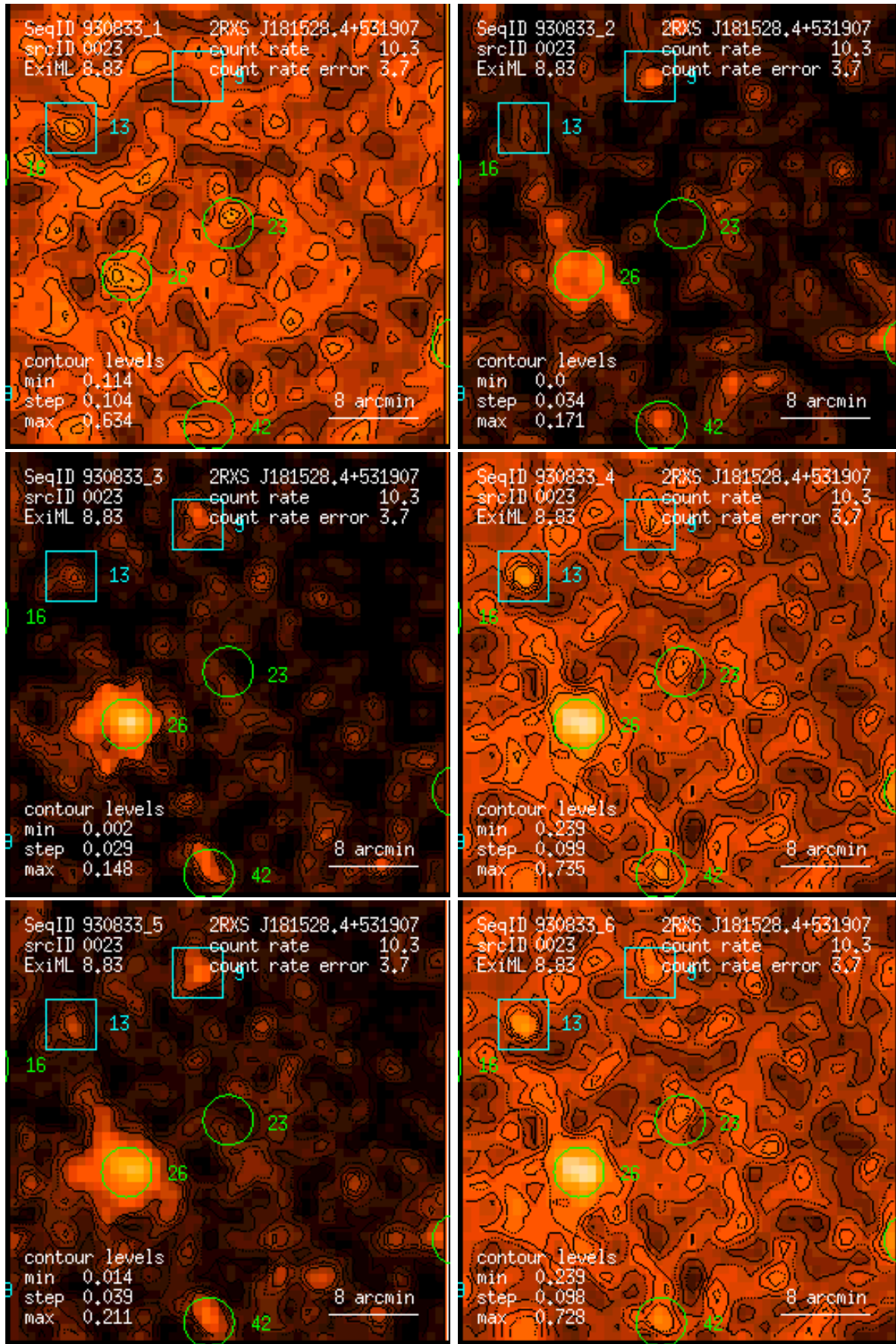
Figure 23: RASS 930833: detection 0023: band rate images, Gaussian filter: (1) PSPC channels 11 – 41, (2) 52 – 90, (3) 91 – 201, (4) 11 – 235, (5) 52 – 201, (6) 11 – 201. Broad band rates in counts/ks. Band rate contour levels in counts/ks/arcmin 2 .
