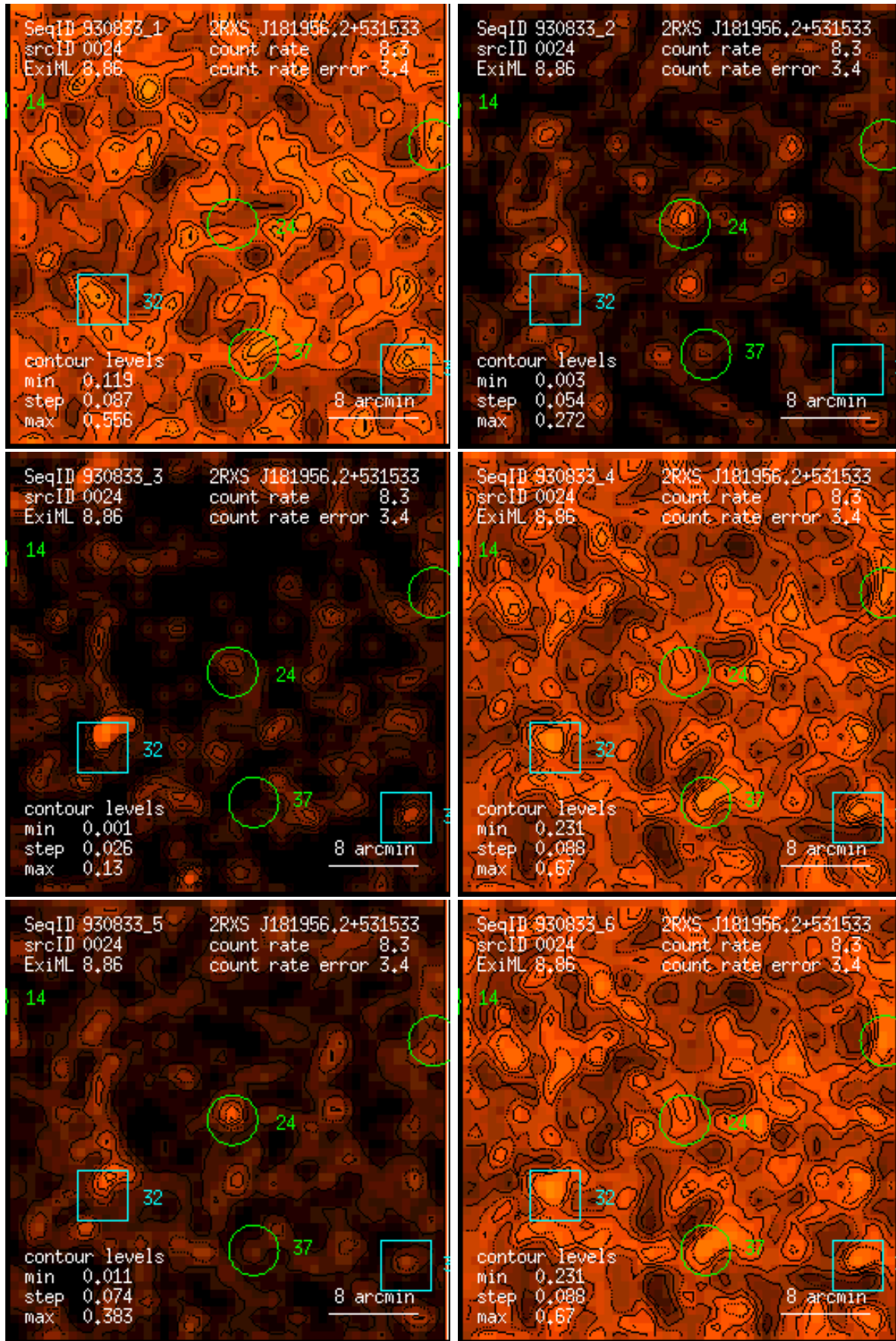
Figure 24: RASS 930833: detection 0024: band rate images, Gaussian filter: (1) PSPC channels 11 – 41, (2) 52 – 90, (3) 91 – 201, (4) 11 – 235, (5) 52 – 201, (6) 11 – 201. Broad band rates in counts/ks. Band rate contour levels in counts/ks/arcmin 2 .
