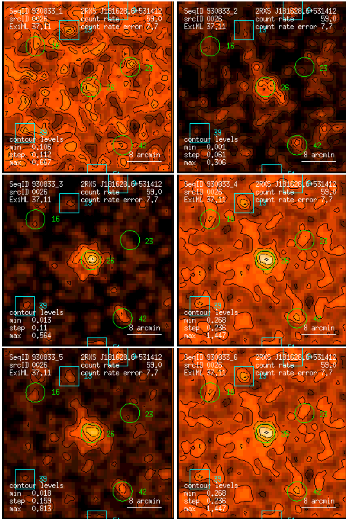
Figure 26: RASS 930833: detection 0026: band rate images, Gaussian filter: (1) PSPC channels 11 – 41, (2) 52 – 90, (3) 91 – 201, (4) 11 – 235, (5) 52 – 201, (6) 11 – 201. Broad band rates in counts/ks. Band rate contour levels in counts/ks/arcmin 2 .
