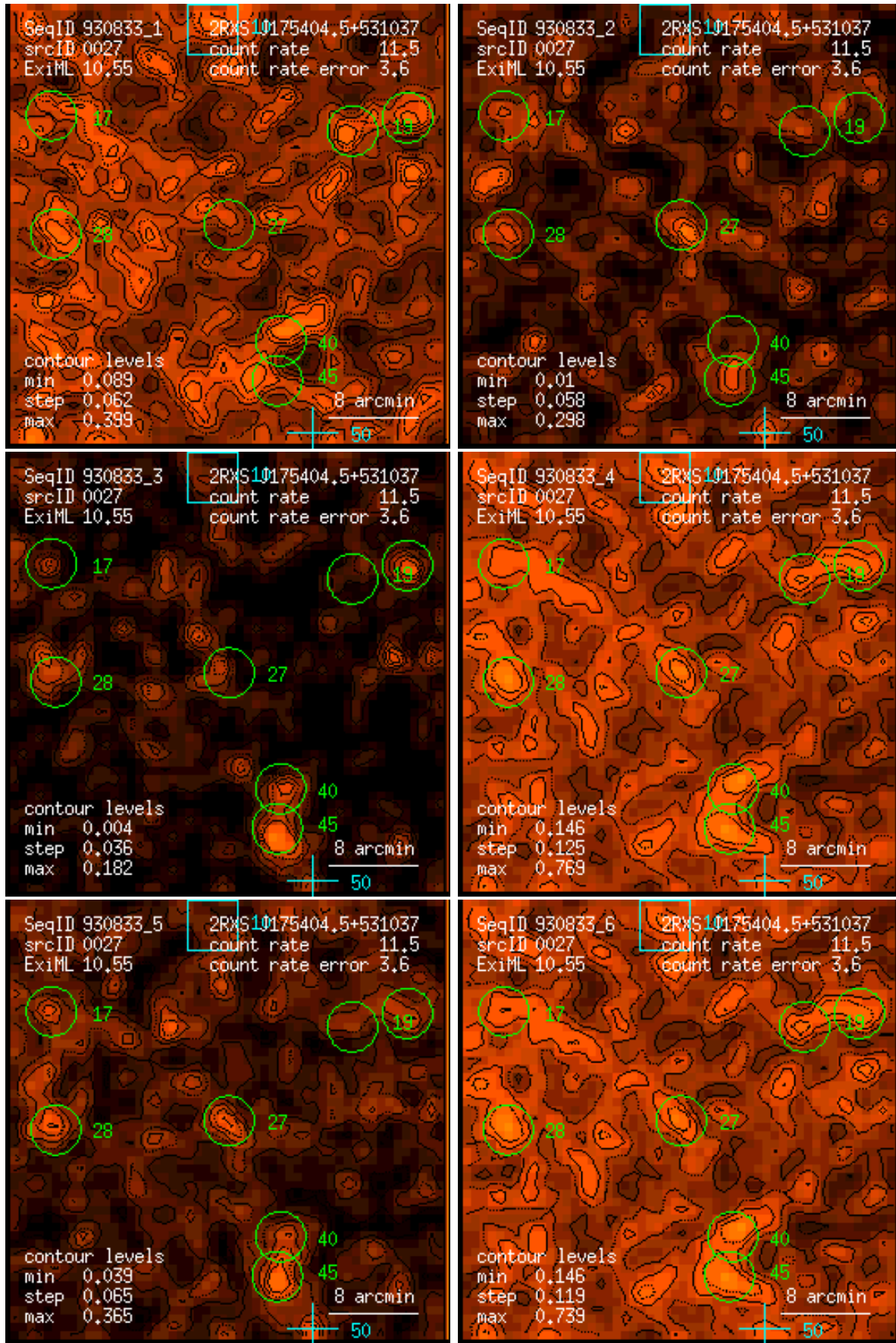
Figure 27: RASS 930833: detection 0027: band rate images, Gaussian filter: (1) PSPC channels 11 – 41, (2) 52 – 90, (3) 91 – 201, (4) 11 – 235, (5) 52 – 201, (6) 11 – 201. Broad band rates in counts/ks. Band rate contour levels in counts/ks/arcmin 2 .
