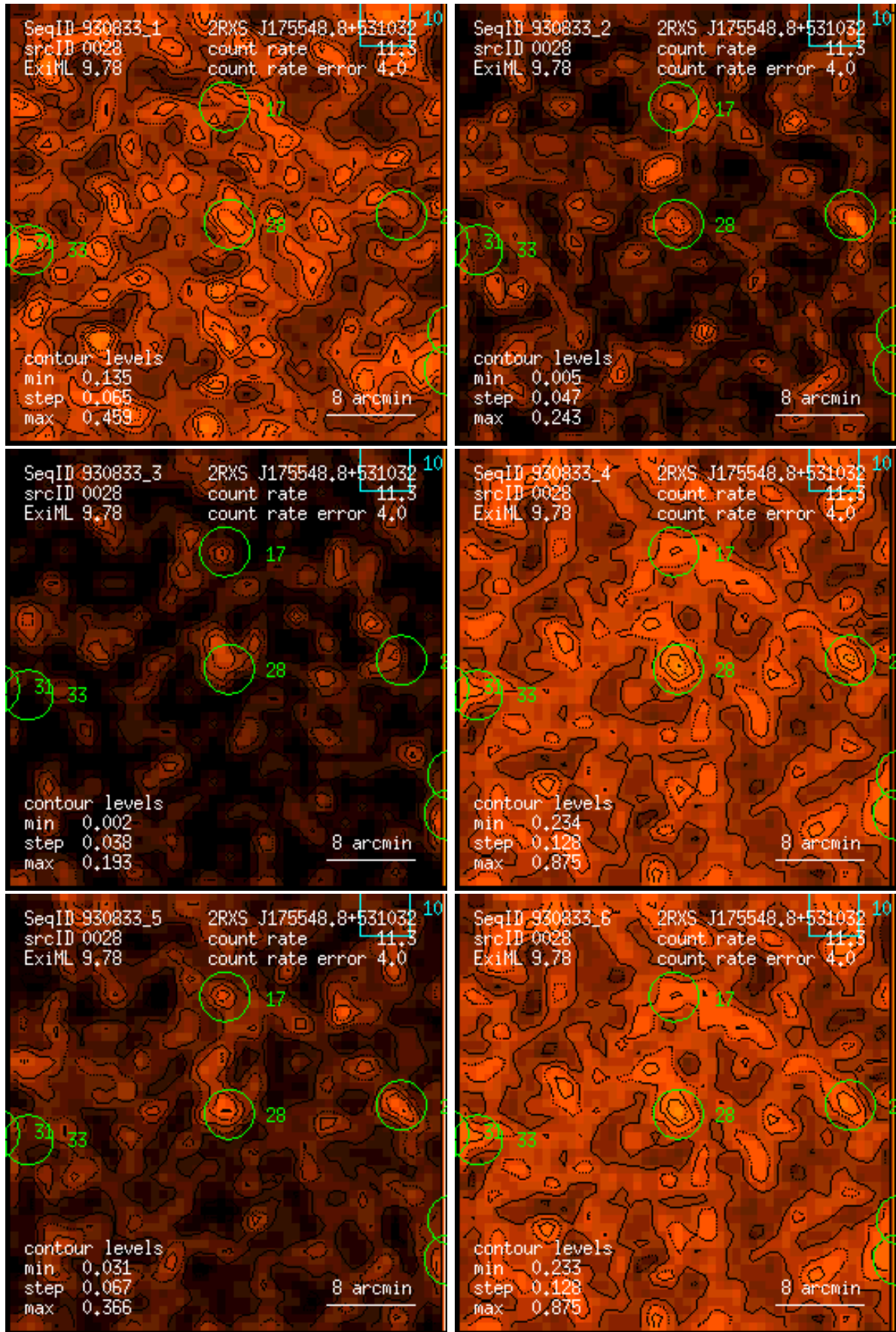
Figure 28: RASS 930833: detection 0028: band rate images, Gaussian filter: (1) PSPC channels 11 – 41, (2) 52 – 90, (3) 91 – 201, (4) 11 – 235, (5) 52 – 201, (6) 11 – 201. Broad band rates in counts/ks. Band rate contour levels in counts/ks/arcmin 2 .
