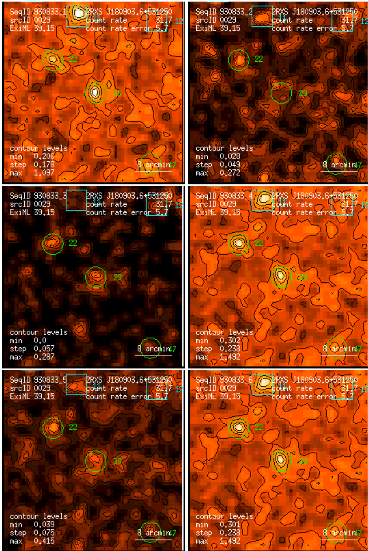
Figure 29: RASS 930833: detection 0029: band rate images, Gaussian filter: (1) PSPC channels 11 – 41, (2) 52 – 90, (3) 91 – 201, (4) 11 – 235, (5) 52 – 201, (6) 11 – 201. Broad band rates in counts/ks. Band rate contour levels in counts/ks/arcmin 2 .
