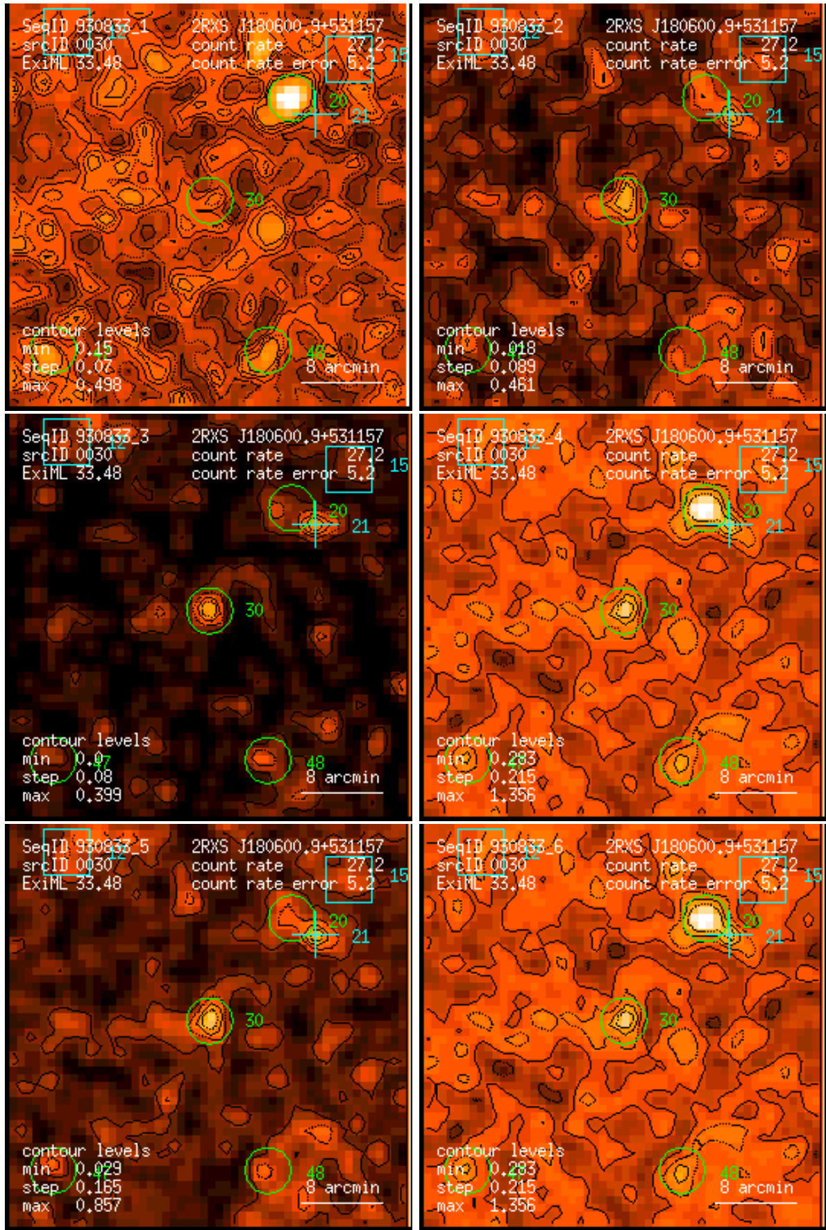
Figure 30: RASS 930833: detection 0030: band rate images, Gaussian filter: (1) PSPC channels 11 – 41, (2) 52 – 90, (3) 91 – 201, (4) 11 – 235, (5) 52 – 201, (6) 11 – 201. Broad band rates in counts/ks. Band rate contour levels in counts/ks/arcmin 2 .
