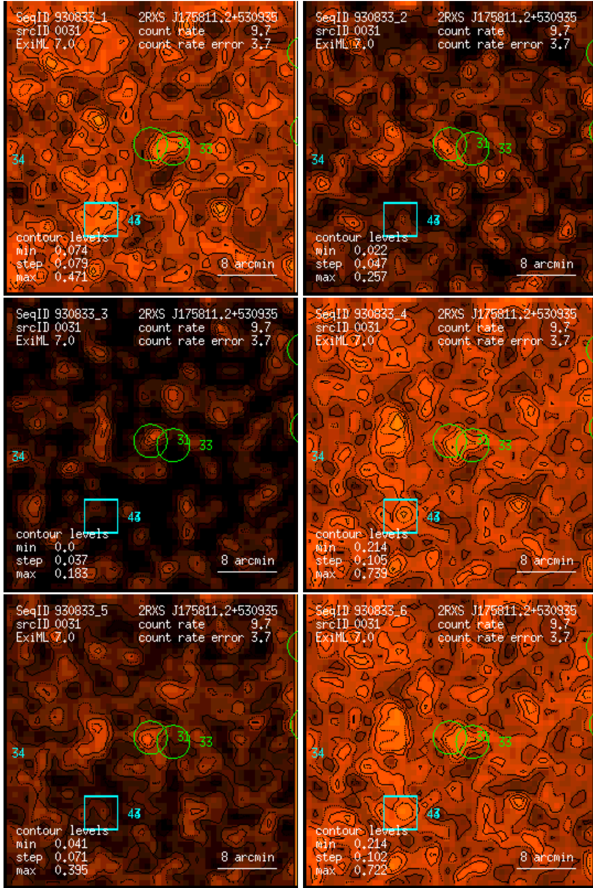
Figure 31: RASS 930833: detection 0031: band rate images, Gaussian filter: (1) PSPC channels 11 – 41, (2) 52 – 90, (3) 91 – 201, (4) 11 – 235, (5) 52 – 201, (6) 11 – 201. Broad band rates in counts/ks. Band rate contour levels in counts/ks/arcmin 2 .
