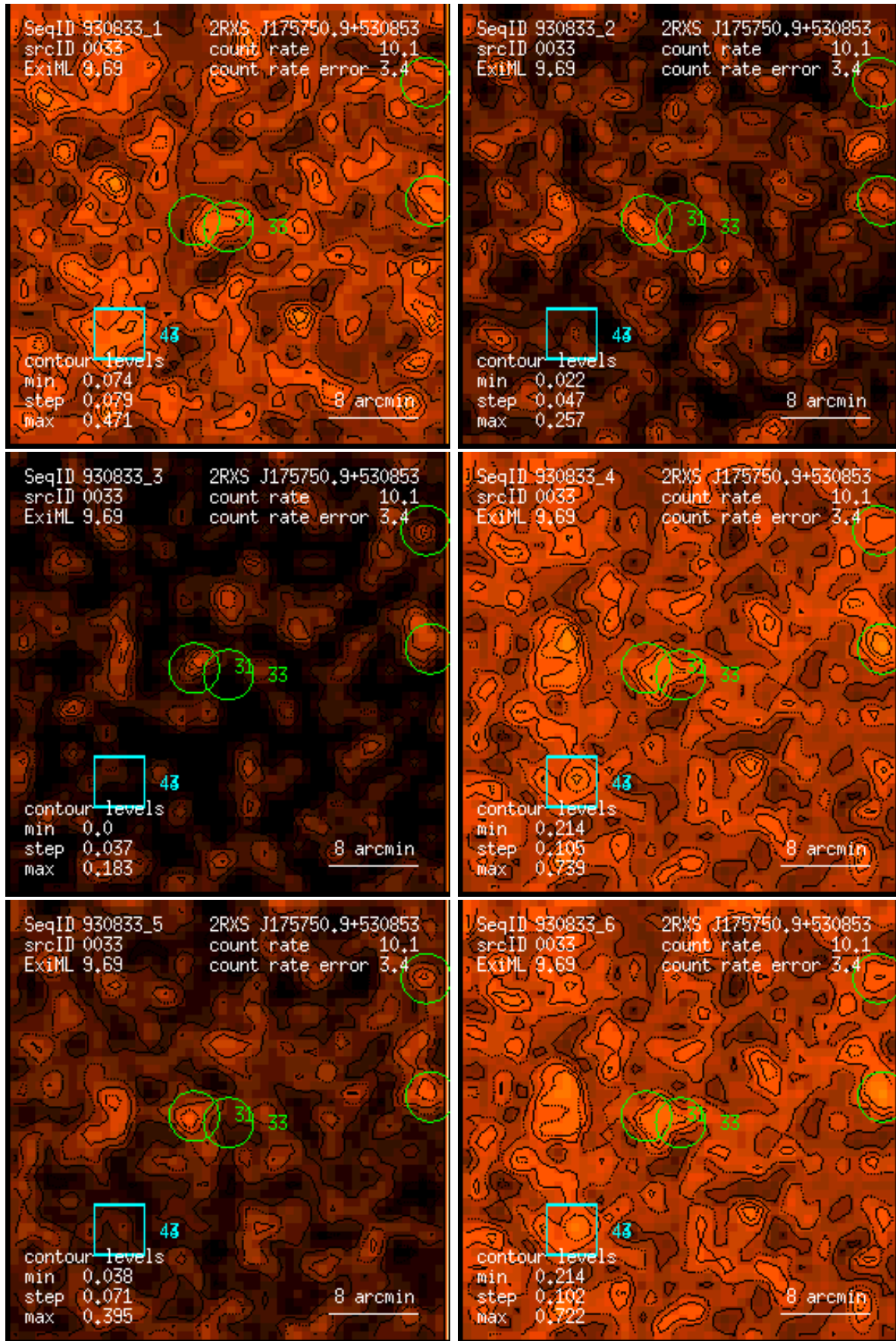
Figure 33: RASS 930833: detection 0033: band rate images, Gaussian filter: (1) PSPC channels 11 – 41, (2) 52 – 90, (3) 91 – 201, (4) 11 – 235, (5) 52 – 201, (6) 11 – 201. Broad band rates in counts/ks. Band rate contour levels in counts/ks/arcmin 2 .
