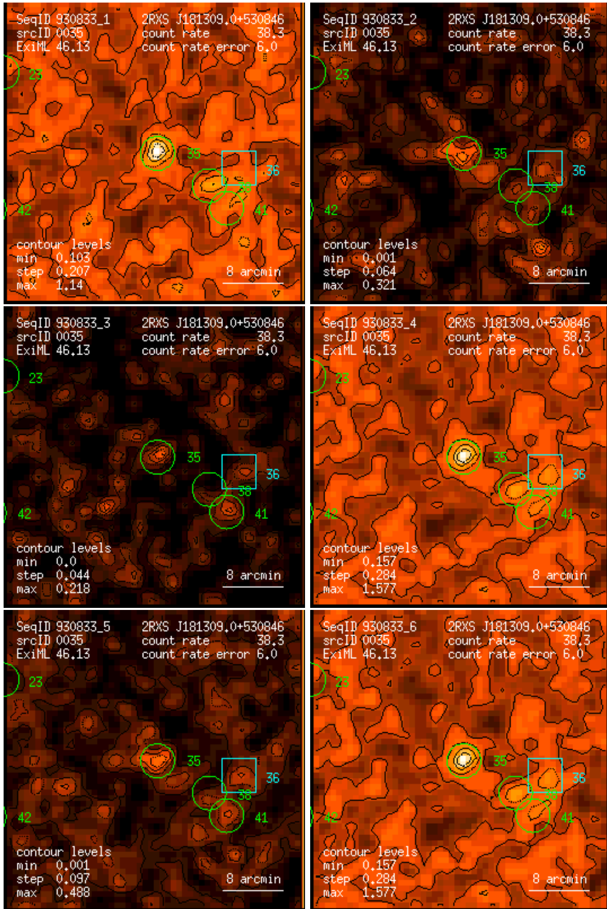
Figure 35: RASS 930833: detection 0035: band rate images, Gaussian filter: (1) PSPC channels 11 – 41, (2) 52 – 90, (3) 91 – 201, (4) 11 – 235, (5) 52 – 201, (6) 11 – 201. Broad band rates in counts/ks. Band rate contour levels in counts/ks/arcmin 2 .
