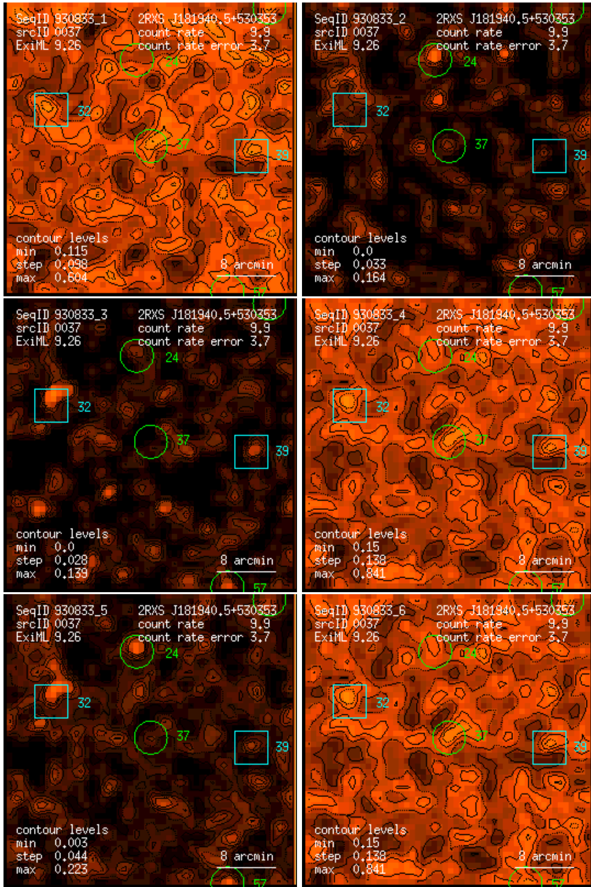
Figure 37: RASS 930833: detection 0037: band rate images, Gaussian filter: (1) PSPC channels 11 – 41, (2) 52 – 90, (3) 91 – 201, (4) 11 – 235, (5) 52 – 201, (6) 11 – 201. Broad band rates in counts/ks. Band rate contour levels in counts/ks/arcmin 2 .
