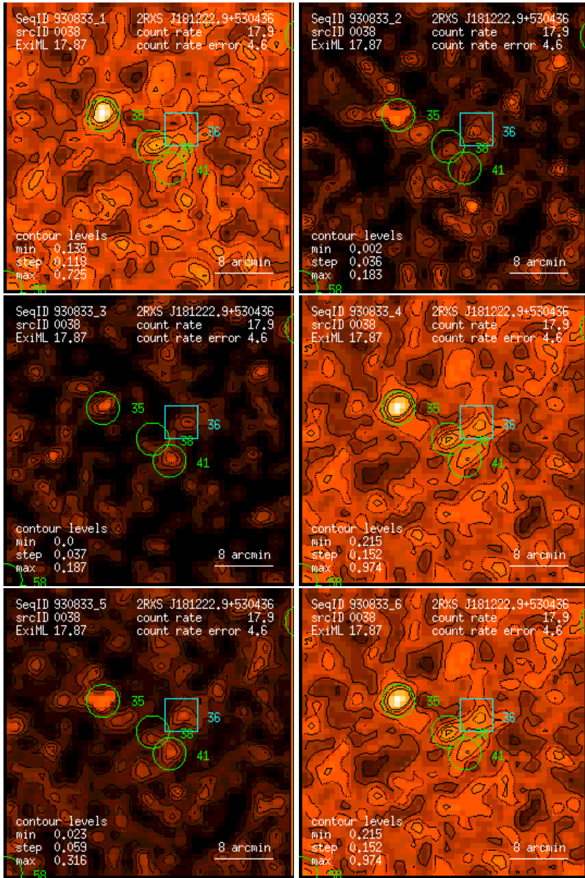
Figure 38: RASS 930833: detection 0038: band rate images, Gaussian filter: (1) PSPC channels 11 – 41, (2) 52 – 90, (3) 91 – 201, (4) 11 – 235, (5) 52 – 201, (6) 11 – 201. Broad band rates in counts/ks. Band rate contour levels in counts/ks/arcmin 2 .
