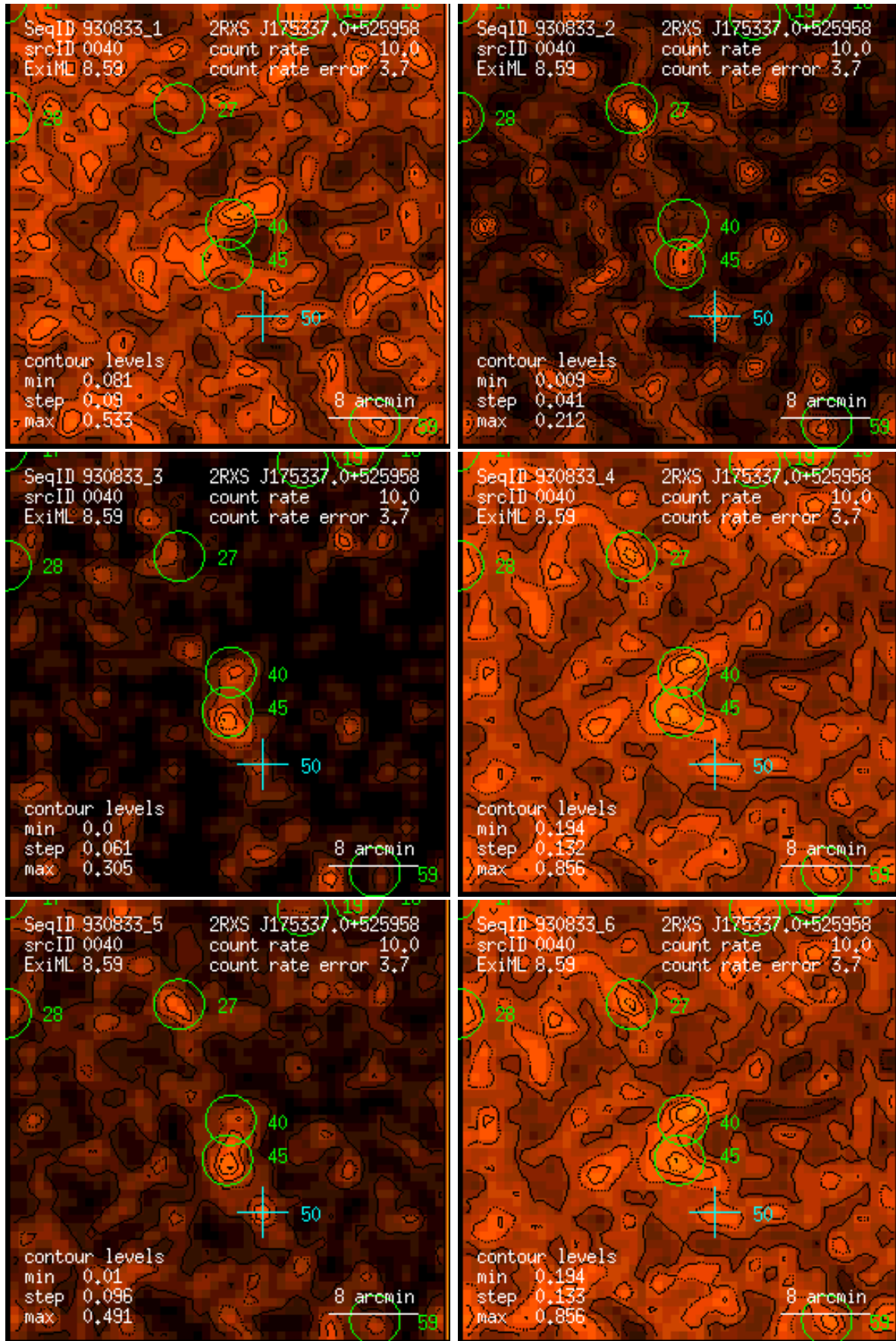
Figure 40: RASS 930833: detection 0040: band rate images, Gaussian filter: (1) PSPC channels 11 – 41, (2) 52 – 90, (3) 91 – 201, (4) 11 – 235, (5) 52 – 201, (6) 11 – 201. Broad band rates in counts/ks. Band rate contour levels in counts/ks/arcmin 2 .
