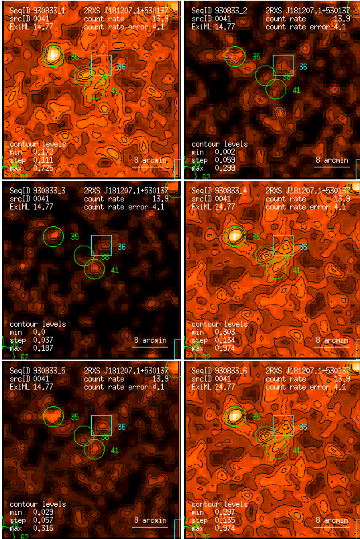
Figure 41: RASS 930833: detection 0041: band rate images, Gaussian filter: (1) PSPC channels 11 – 41, (2) 52 – 90, (3) 91 – 201, (4) 11 – 235, (5) 52 – 201, (6) 11 – 201. Broad band rates in counts/ks. Band rate contour levels in counts/ks/arcmin 2 .
