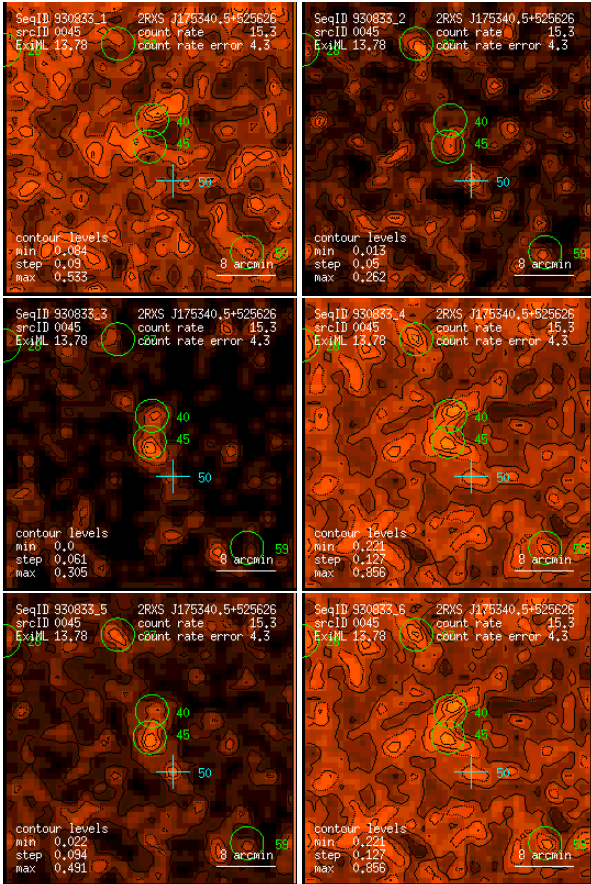
Figure 45: RASS 930833: detection 0045: band rate images, Gaussian filter: (1) PSPC channels 11 – 41, (2) 52 – 90, (3) 91 – 201, (4) 11 – 235, (5) 52 – 201, (6) 11 – 201. Broad band rates in counts/ks. Band rate contour levels in counts/ks/arcmin 2 .
