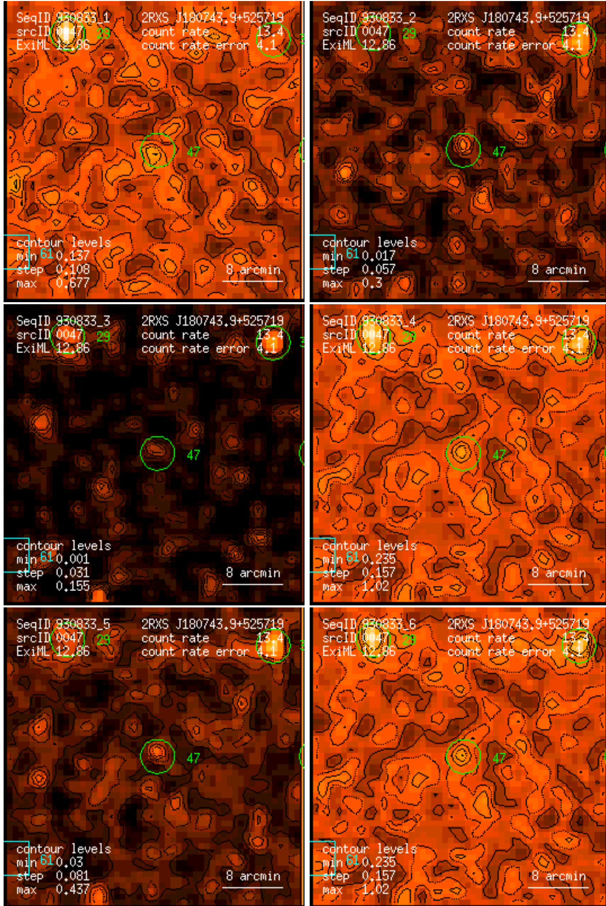
Figure 47: RASS 930833: detection 0047: band rate images, Gaussian filter: (1) PSPC channels 11 – 41, (2) 52 – 90, (3) 91 – 201, (4) 11 – 235, (5) 52 – 201, (6) 11 – 201. Broad band rates in counts/ks. Band rate contour levels in counts/ks/arcmin 2 .
