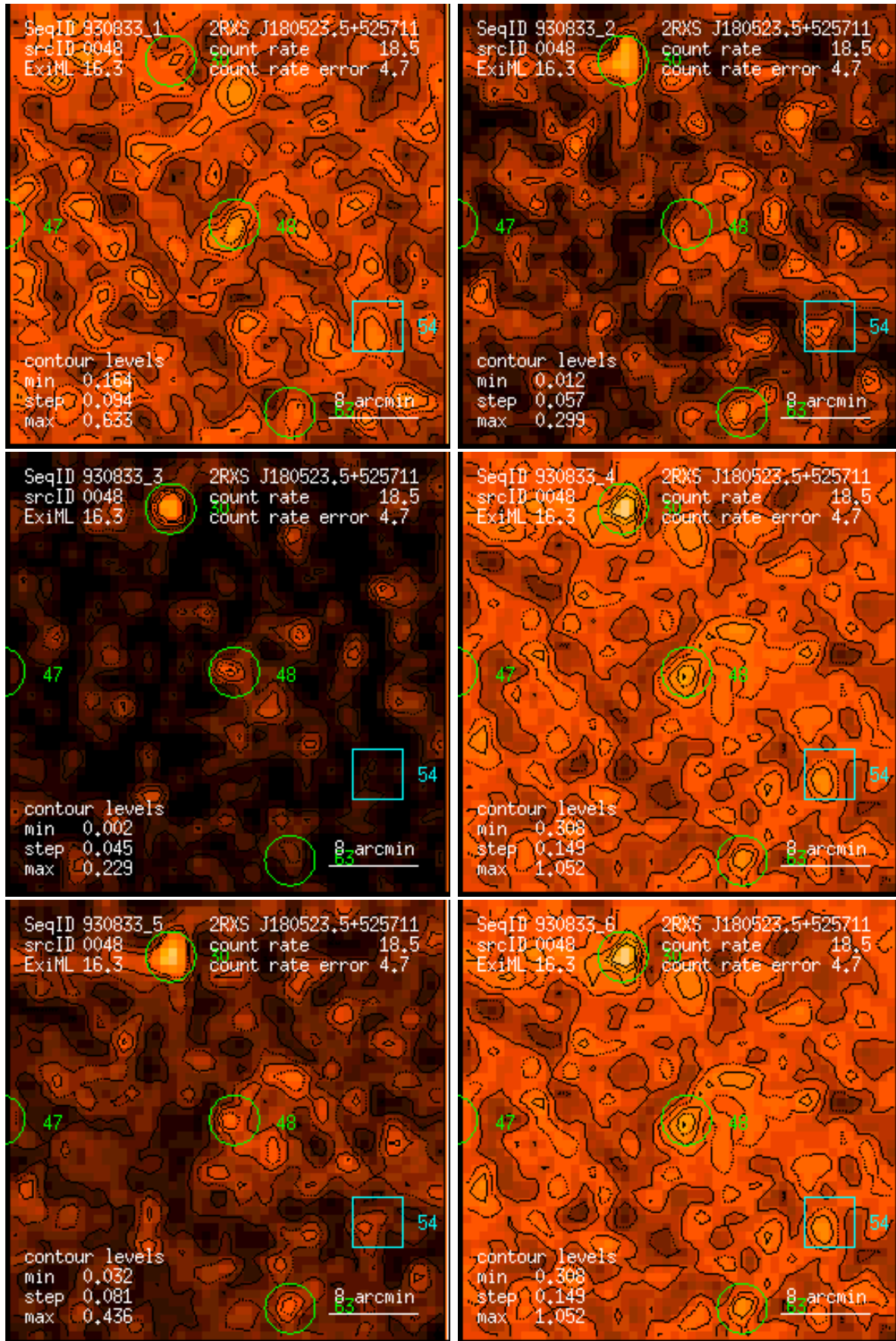
Figure 48: RASS 930833: detection 0048: band rate images, Gaussian filter: (1) PSPC channels 11 – 41, (2) 52 – 90, (3) 91 – 201, (4) 11 – 235, (5) 52 – 201, (6) 11 – 201. Broad band rates in counts/ks. Band rate contour levels in counts/ks/arcmin 2 .
