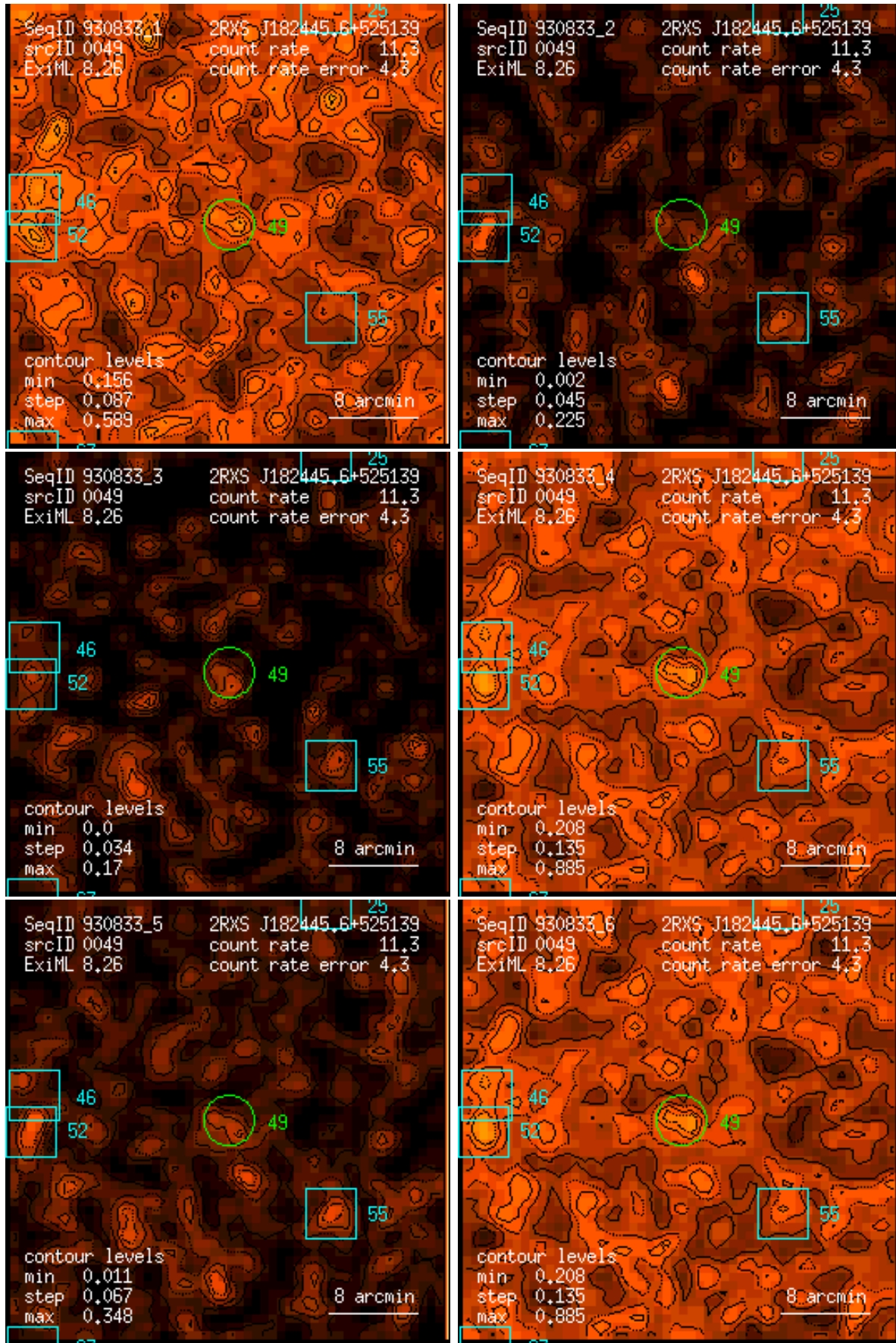
Figure 49: RASS 930833: detection 0049: band rate images, Gaussian filter: (1) PSPC channels 11 – 41, (2) 52 – 90, (3) 91 – 201, (4) 11 – 235, (5) 52 – 201, (6) 11 – 201. Broad band rates in counts/ks. Band rate contour levels in counts/ks/arcmin 2 .
