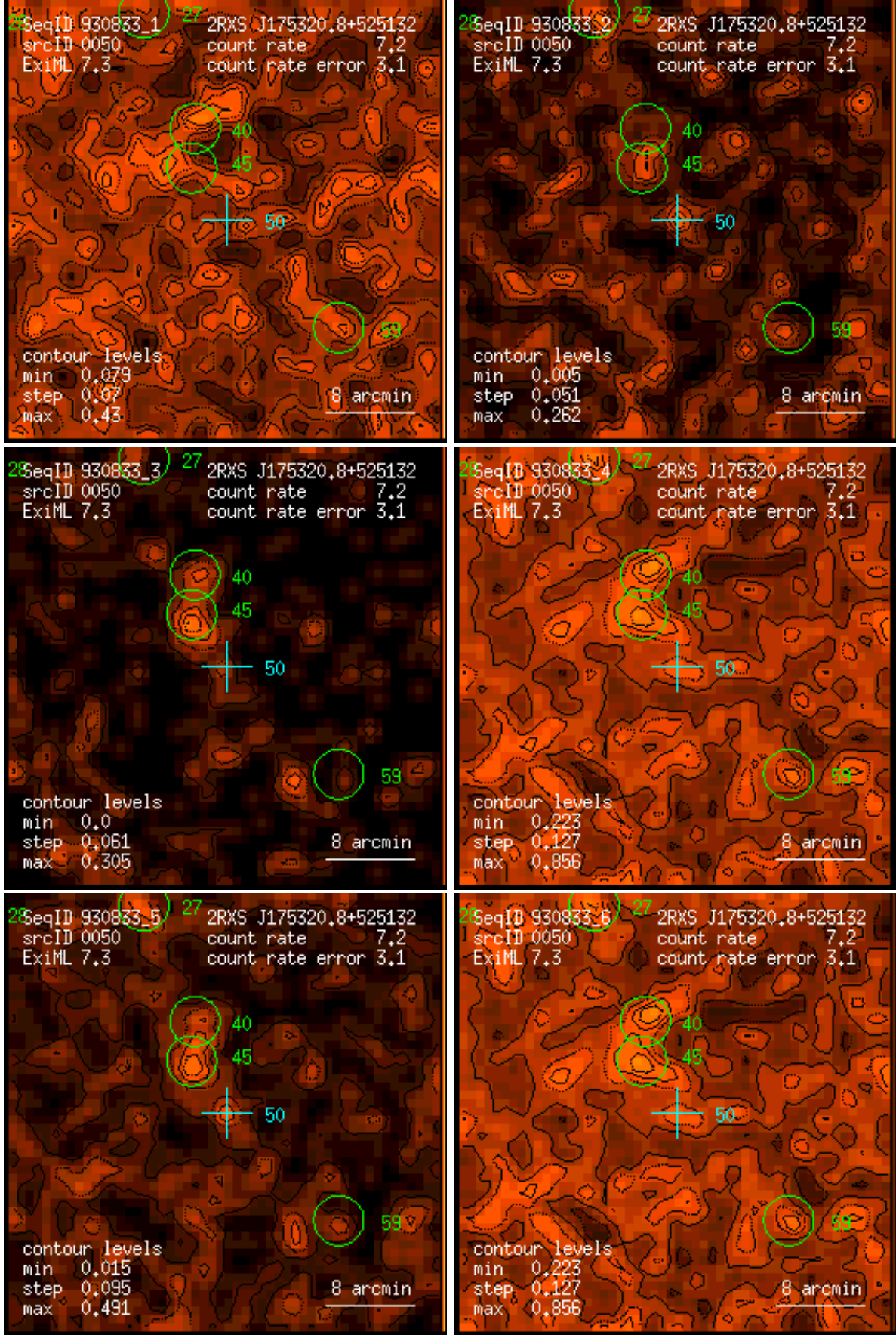
Figure 50: RASS 930833: detection 0050: band rate images, Gaussian filter: (1) PSPC channels 11 – 41, (2) 52 – 90, (3) 91 – 201, (4) 11 – 235, (5) 52 – 201, (6) 11 – 201. Broad band rates in counts/ks. Band rate contour levels in counts/ks/arcmin 2 .
