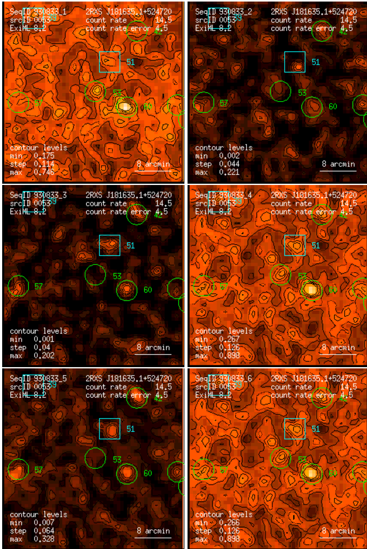
Figure 53: RASS 930833: detection 0053: band rate images, Gaussian filter: (1) PSPC channels 11 – 41, (2) 52 – 90, (3) 91 – 201, (4) 11 – 235, (5) 52 – 201, (6) 11 – 201. Broad band rates in counts/ks. Band rate contour levels in counts/ks/arcmin 2 .
