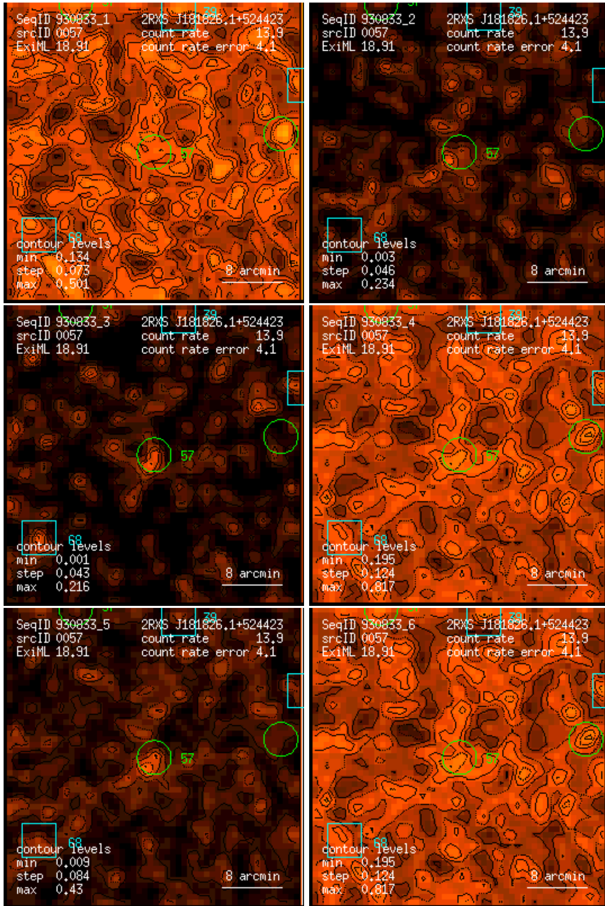
Figure 57: RASS 930833: detection 0057: band rate images, Gaussian filter: (1) PSPC channels 11 – 41, (2) 52 – 90, (3) 91 – 201, (4) 11 – 235, (5) 52 – 201, (6) 11 – 201. Broad band rates in counts/ks. Band rate contour levels in counts/ks/arcmin 2 .
