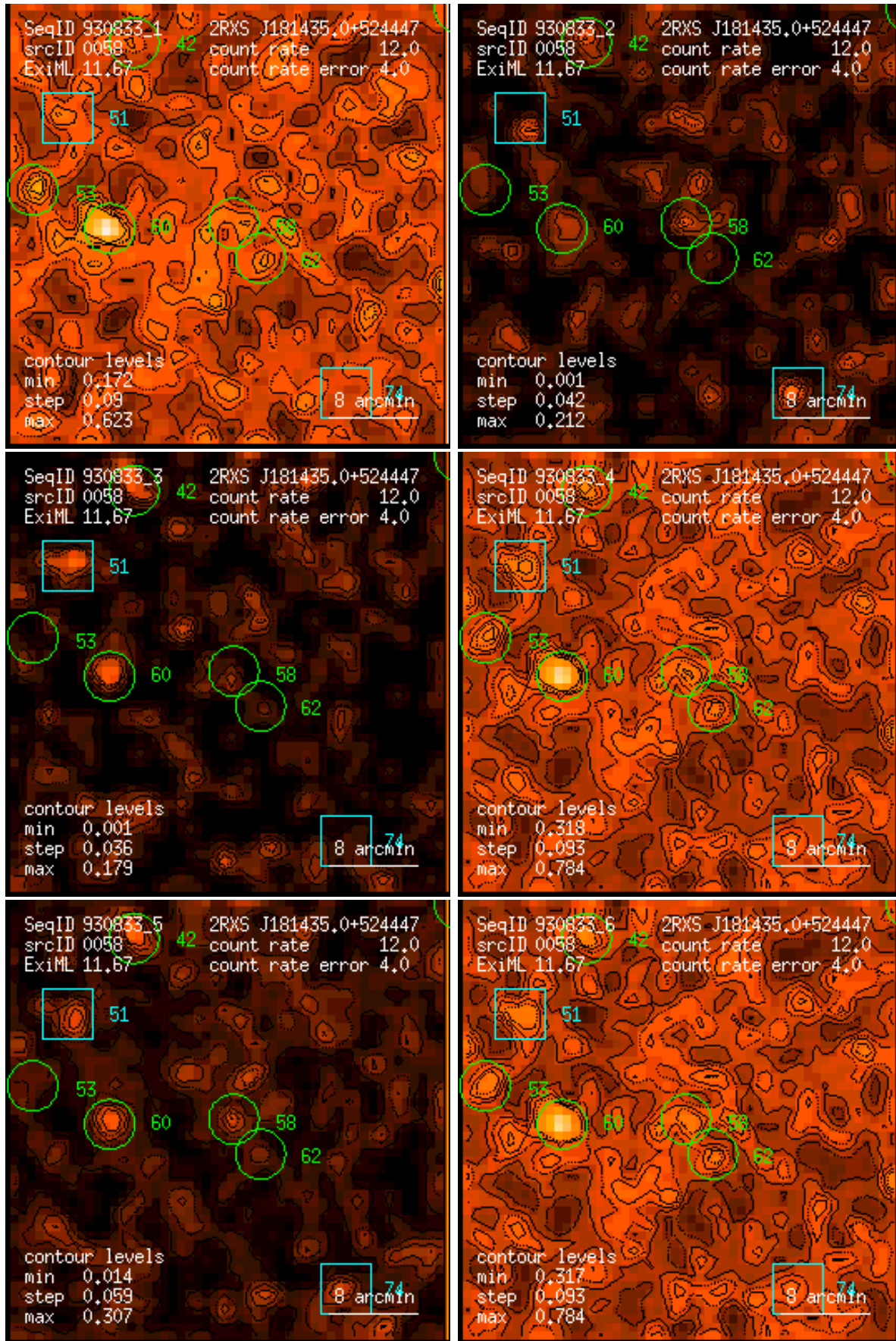
Figure 58: RASS 930833: detection 0058: band rate images, Gaussian filter: (1) PSPC channels 11 – 41, (2) 52 – 90, (3) 91 – 201, (4) 11 – 235, (5) 52 – 201, (6) 11 – 201. Broad band rates in counts/ks. Band rate contour levels in counts/ks/arcmin 2 .
