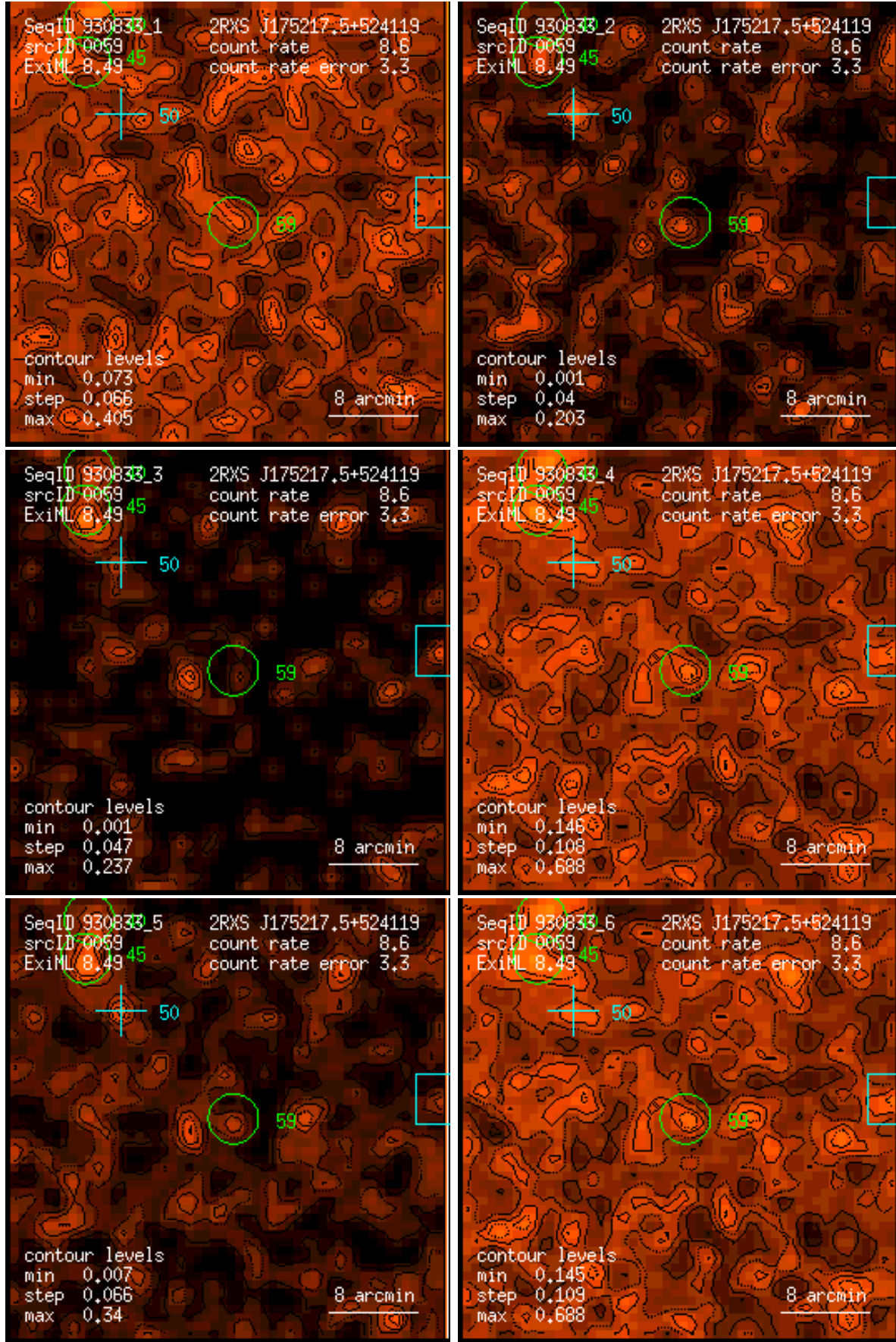
Figure 59: RASS 930833: detection 0059: band rate images, Gaussian filter: (1) PSPC channels 11 – 41, (2) 52 – 90, (3) 91 – 201, (4) 11 – 235, (5) 52 – 201, (6) 11 – 201. Broad band rates in counts/ks. Band rate contour levels in counts/ks/arcmin 2 .
