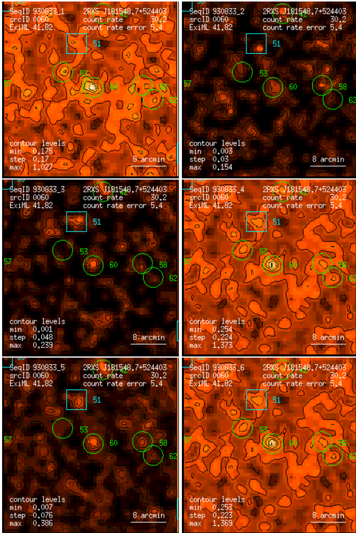
Figure 60: RASS 930833: detection 0060: band rate images, Gaussian filter: (1) PSPC channels 11 – 41, (2) 52 – 90, (3) 91 – 201, (4) 11 – 235, (5) 52 – 201, (6) 11 – 201. Broad band rates in counts/ks. Band rate contour levels in counts/ks/arcmin 2 .
