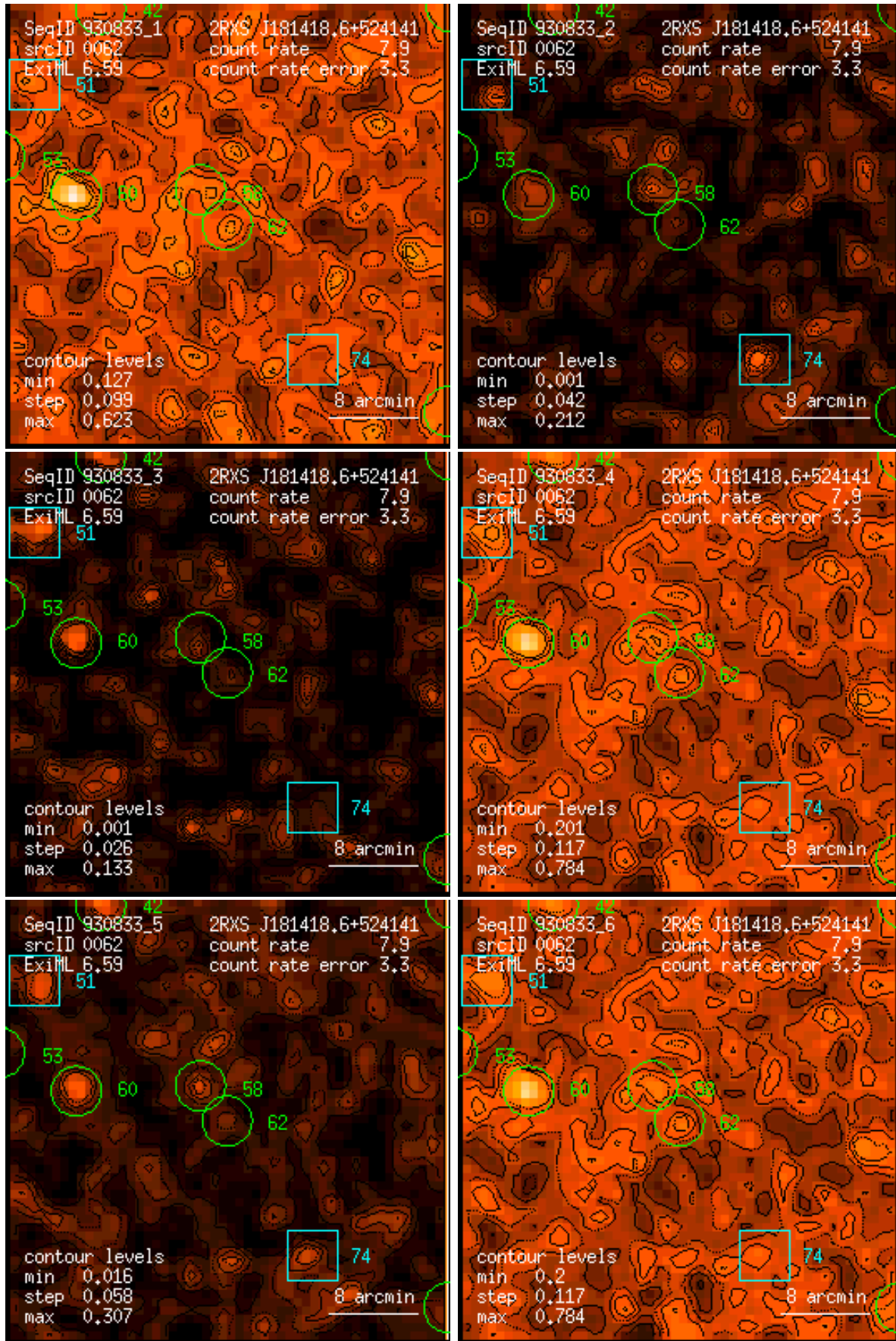
Figure 62: RASS 930833: detection 0062: band rate images, Gaussian filter: (1) PSPC channels 11 – 41, (2) 52 – 90, (3) 91 – 201, (4) 11 – 235, (5) 52 – 201, (6) 11 – 201. Broad band rates in counts/ks. Band rate contour levels in counts/ks/arcmin 2 .
