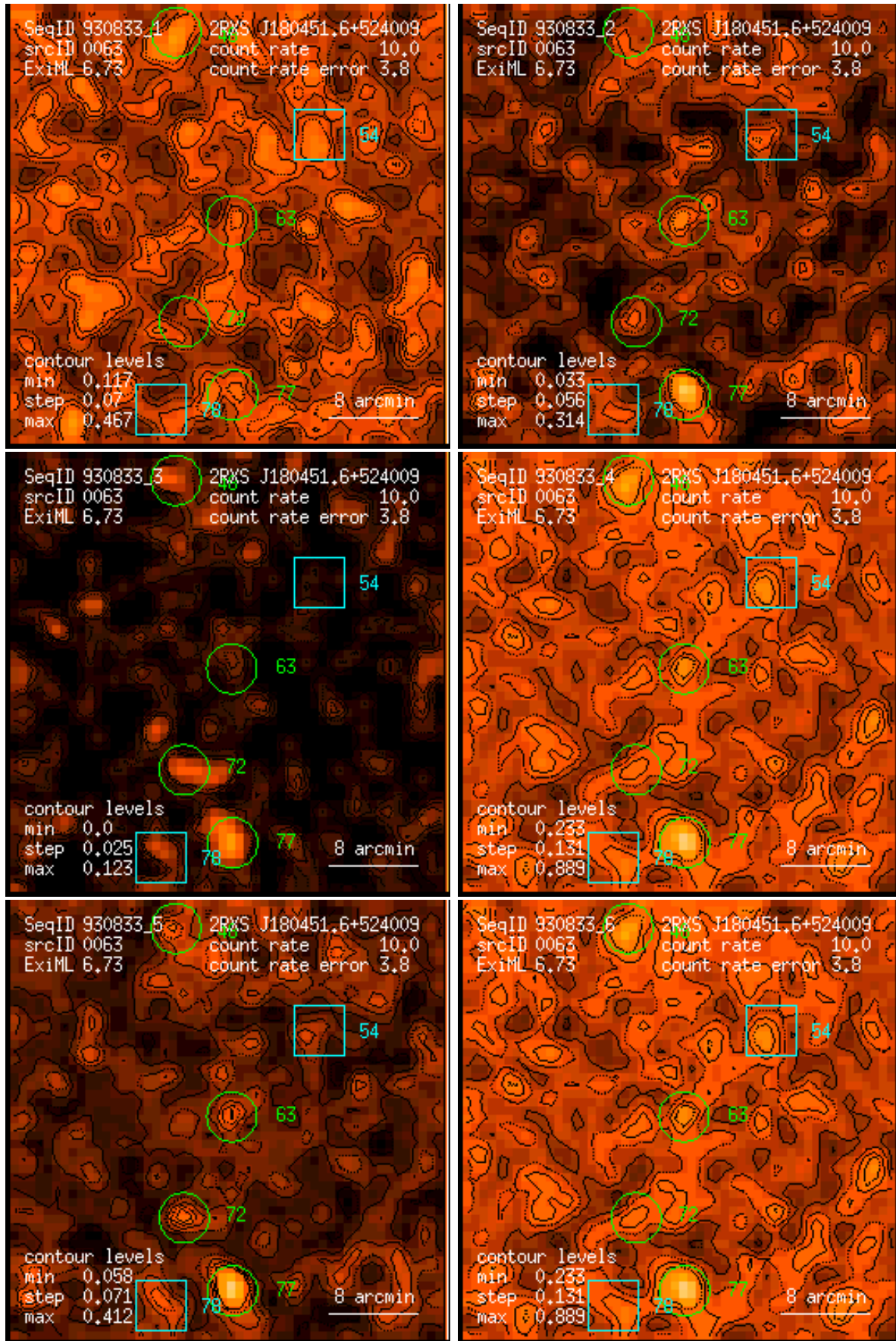
Figure 63: RASS 930833: detection 0063: band rate images, Gaussian filter: (1) PSPC channels 11 – 41, (2) 52 – 90, (3) 91 – 201, (4) 11 – 235, (5) 52 – 201, (6) 11 – 201. Broad band rates in counts/ks. Band rate contour levels in counts/ks/arcmin 2 .
