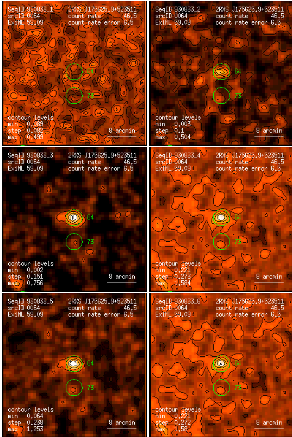
Figure 64: RASS 930833: detection 0064: band rate images, Gaussian filter: (1) PSPC channels 11 – 41, (2) 52 – 90, (3) 91 – 201, (4) 11 – 235, (5) 52 – 201, (6) 11 – 201. Broad band rates in counts/ks. Band rate contour levels in counts/ks/arcmin 2 .
