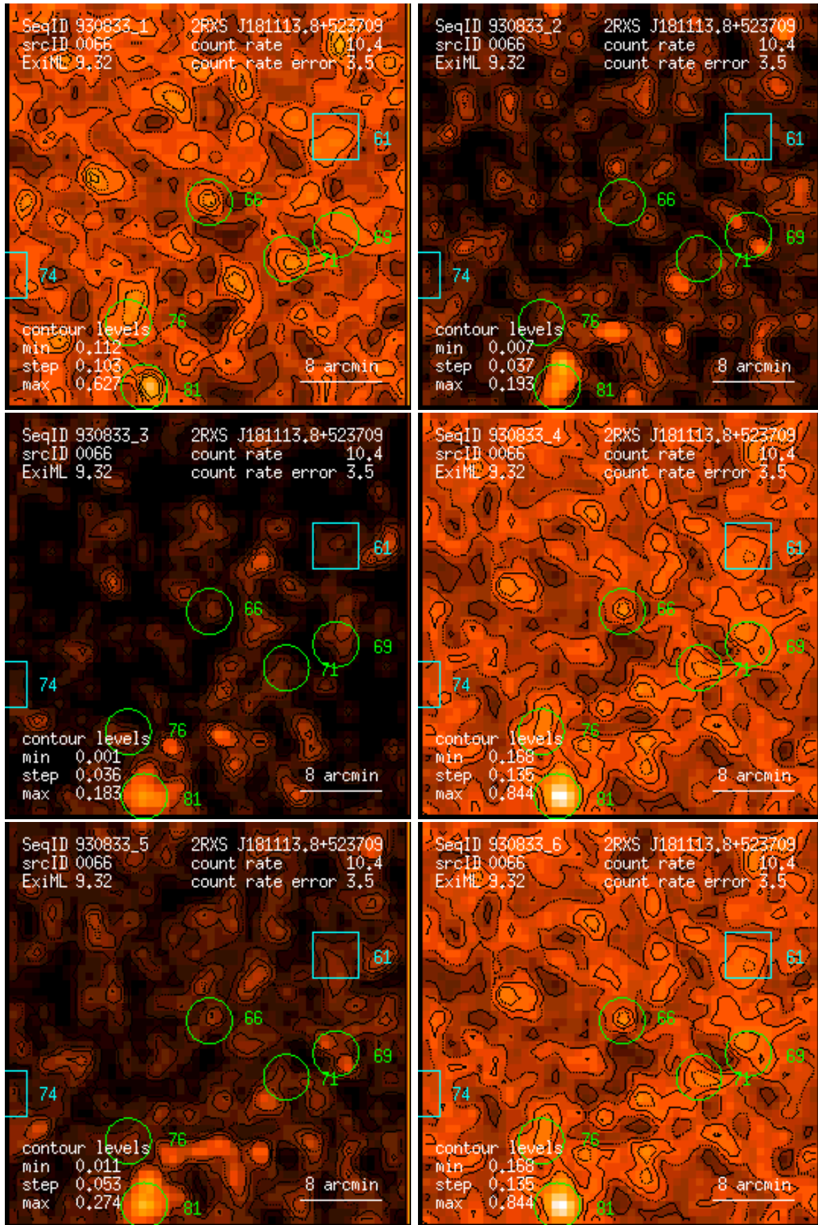
Figure 66: RASS 930833: detection 0066: band rate images, Gaussian filter: (1) PSPC channels 11 – 41, (2) 52 – 90, (3) 91 – 201, (4) 11 – 235, (5) 52 – 201, (6) 11 – 201. Broad band rates in counts/ks. Band rate contour levels in counts/ks/arcmin 2 .
