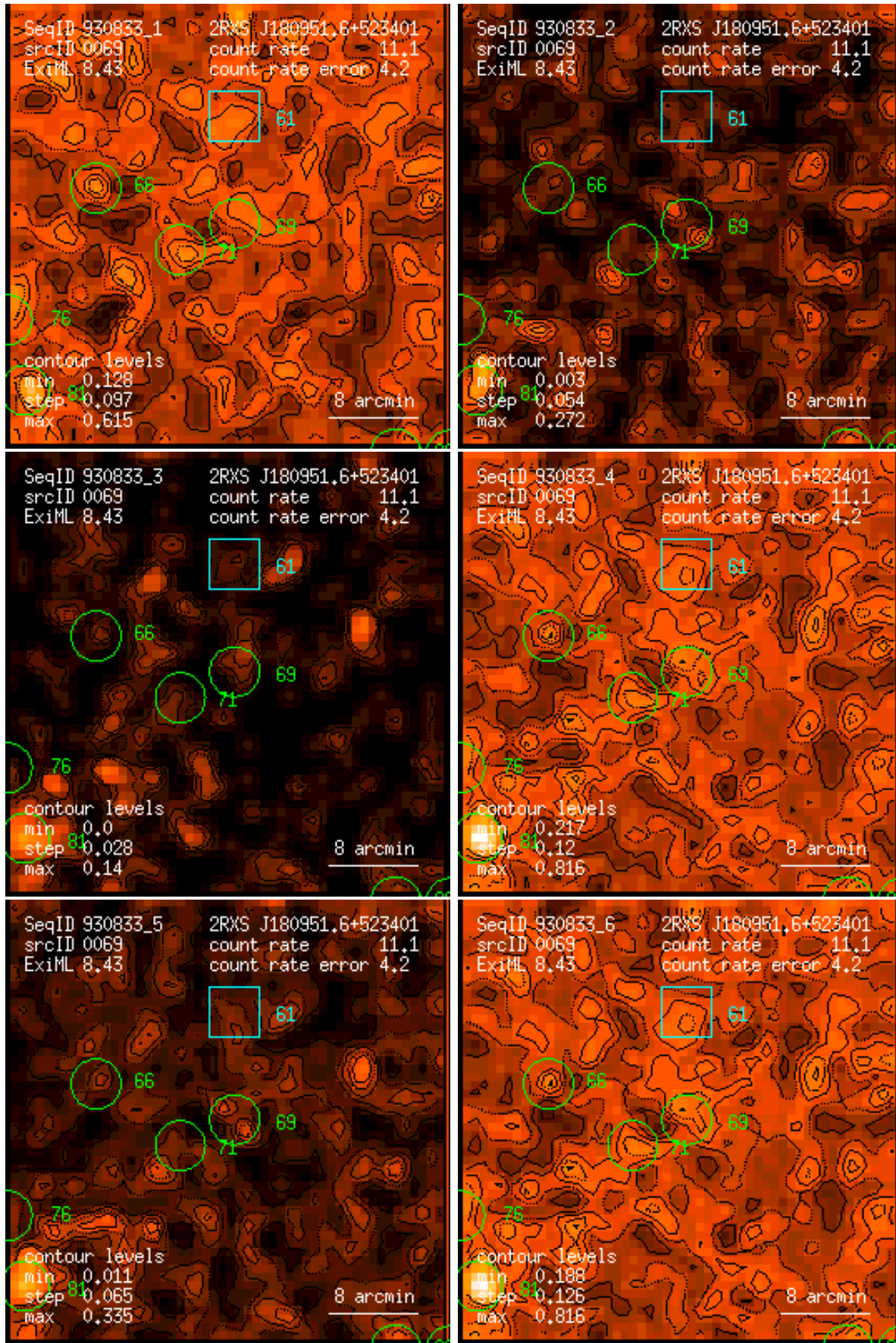
Figure 69: RASS 930833: detection 0069: band rate images, Gaussian filter: (1) PSPC channels 11 – 41, (2) 52 – 90, (3) 91 – 201, (4) 11 – 235, (5) 52 – 201, (6) 11 – 201. Broad band rates in counts/ks. Band rate contour levels in counts/ks/arcmin 2 .
