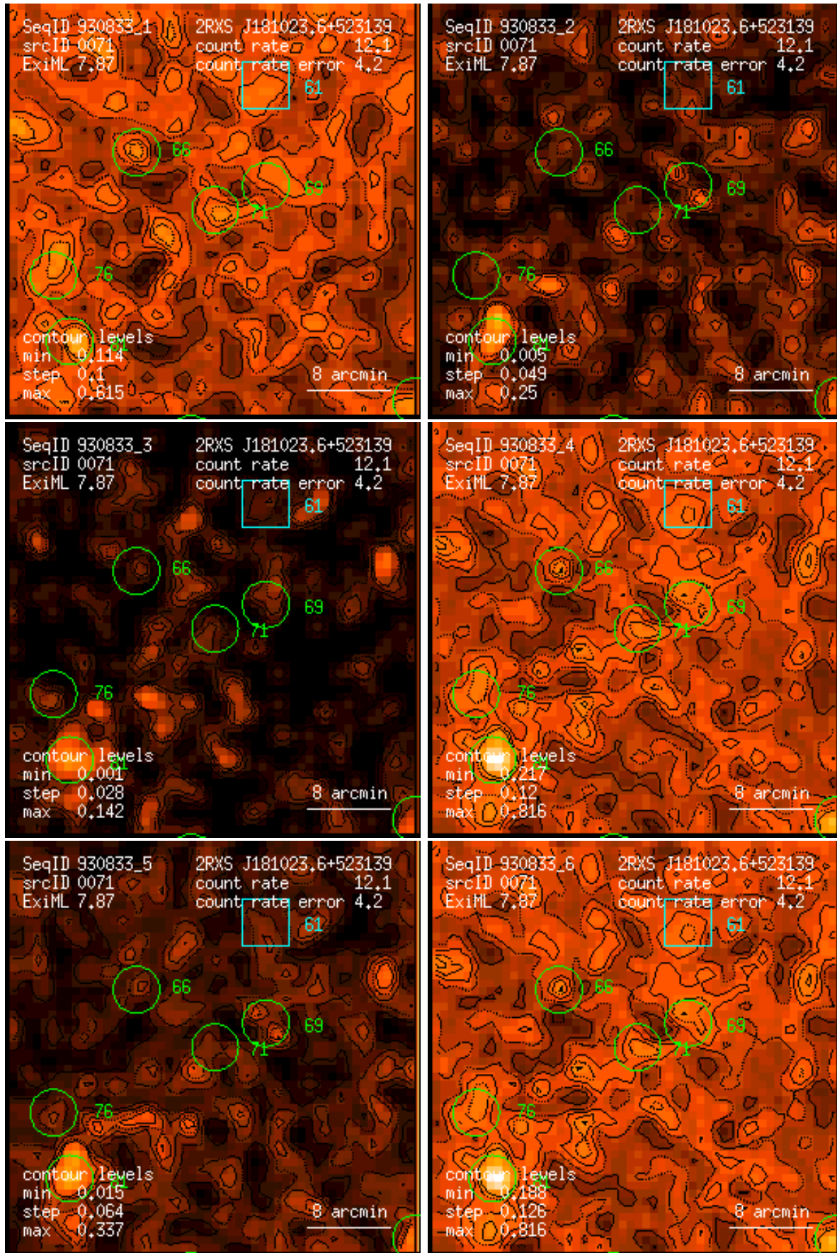
Figure 71: RASS 930833: detection 0071: band rate images, Gaussian filter: (1) PSPC channels 11 – 41, (2) 52 – 90, (3) 91 – 201, (4) 11 – 235, (5) 52 – 201, (6) 11 – 201. Broad band rates in counts/ks. Band rate contour levels in counts/ks/arcmin 2 .
