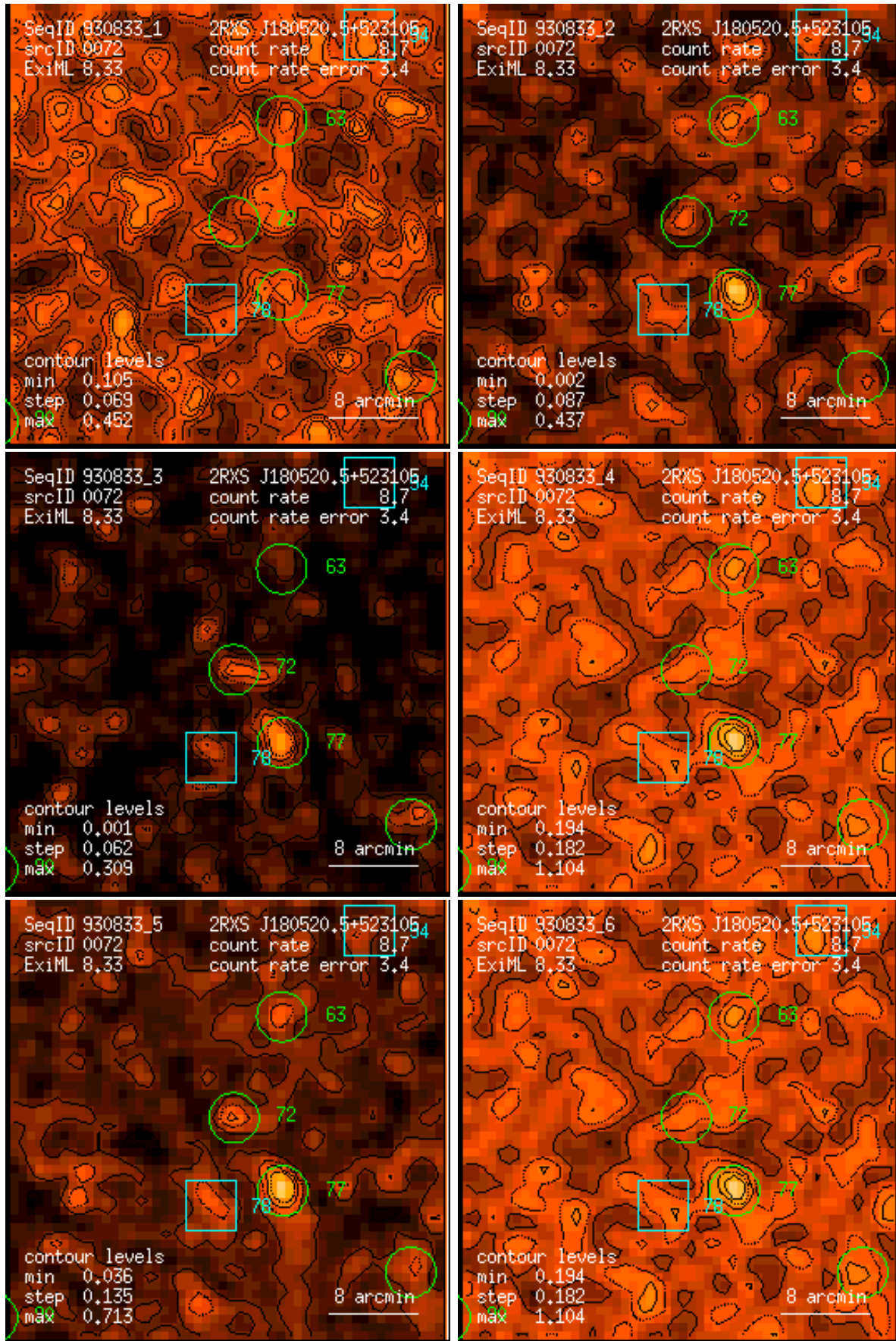
Figure 72: RASS 930833: detection 0072: band rate images, Gaussian filter: (1) PSPC channels 11 – 41, (2) 52 – 90, (3) 91 – 201, (4) 11 – 235, (5) 52 – 201, (6) 11 – 201. Broad band rates in counts/ks. Band rate contour levels in counts/ks/arcmin 2 .
