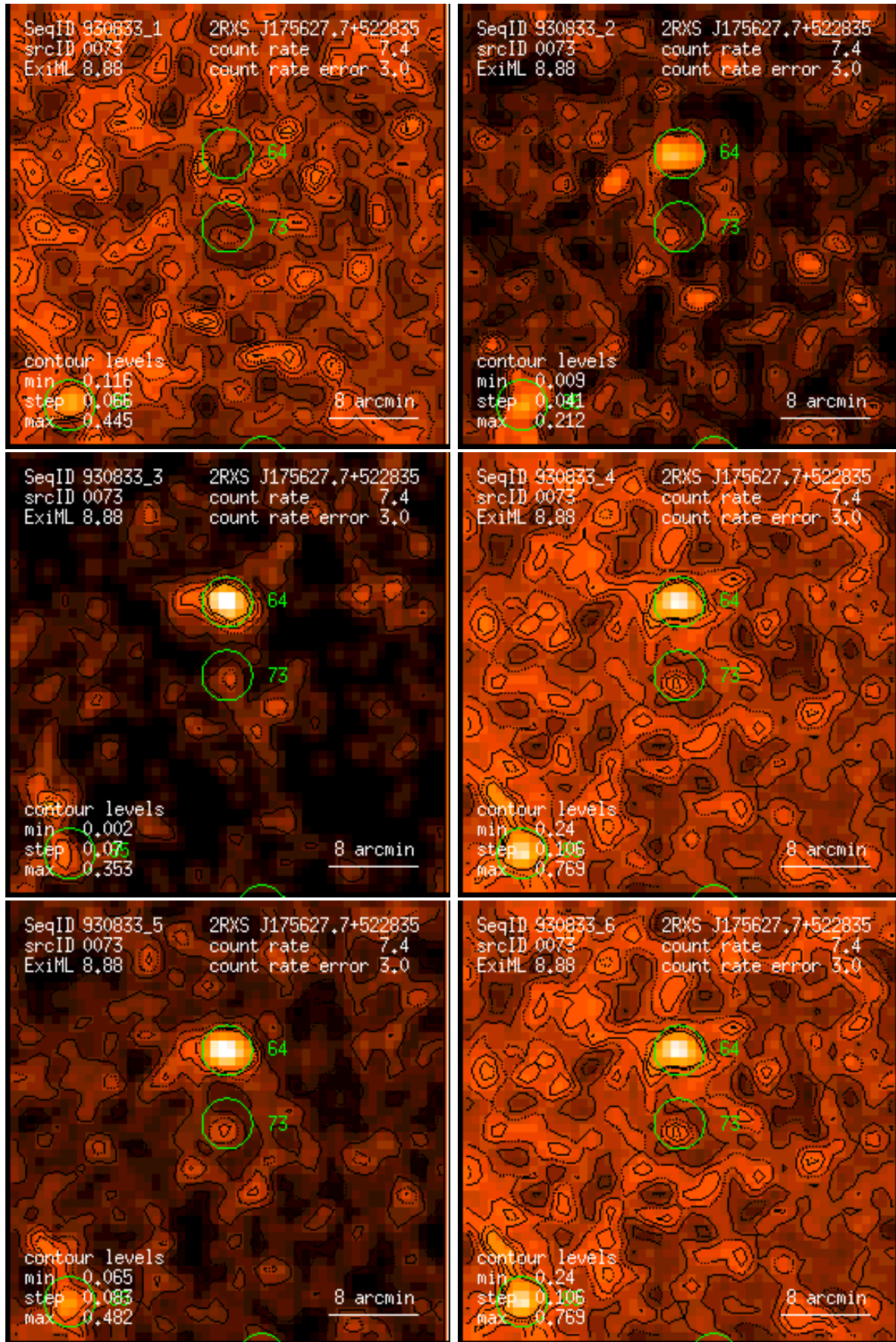
Figure 73: RASS 930833: detection 0073: band rate images, Gaussian filter: (1) PSPC channels 11 – 41, (2) 52 – 90, (3) 91 – 201, (4) 11 – 235, (5) 52 – 201, (6) 11 – 201. Broad band rates in counts/ks. Band rate contour levels in counts/ks/arcmin 2 .
