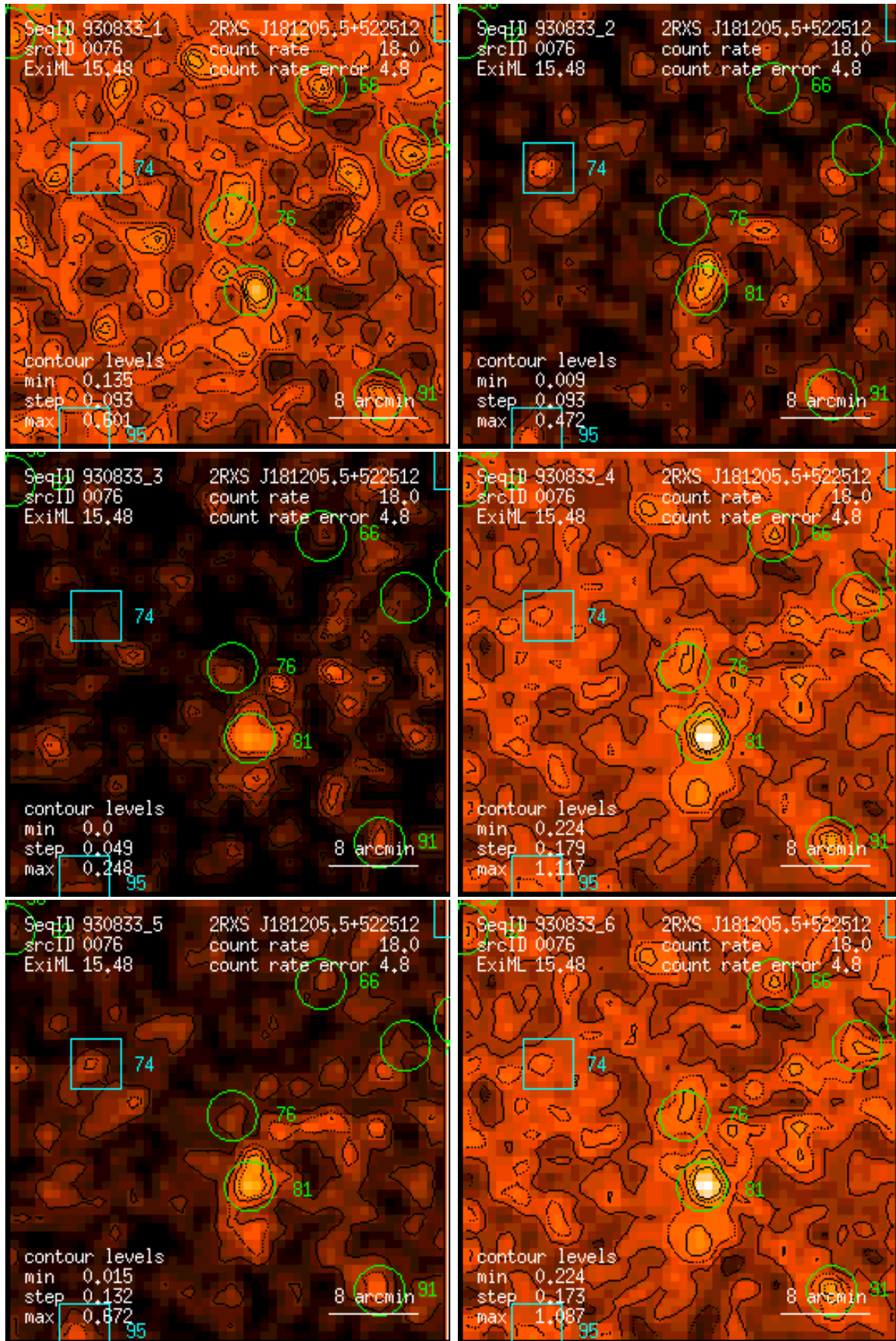
Figure 76: RASS 930833: detection 0076: band rate images, Gaussian filter: (1) PSPC channels 11 – 41, (2) 52 – 90, (3) 91 – 201, (4) 11 – 235, (5) 52 – 201, (6) 11 – 201. Broad band rates in counts/ks. Band rate contour levels in counts/ks/arcmin 2 .
