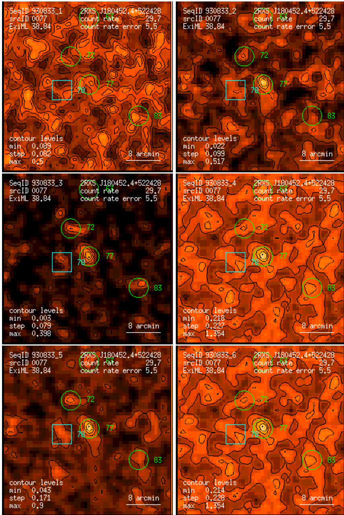
Figure 77: RASS 930833: detection 0077: band rate images, Gaussian filter: (1) PSPC channels 11 – 41, (2) 52 – 90, (3) 91 – 201, (4) 11 – 235, (5) 52 – 201, (6) 11 – 201. Broad band rates in counts/ks. Band rate contour levels in counts/ks/arcmin 2 .
