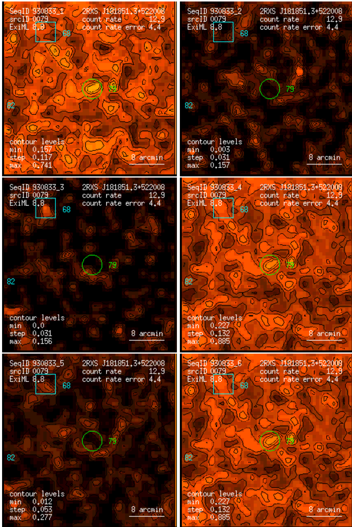
Figure 79: RASS 930833: detection 0079: band rate images, Gaussian filter: (1) PSPC channels 11 – 41, (2) 52 – 90, (3) 91 – 201, (4) 11 – 235, (5) 52 – 201, (6) 11 – 201. Broad band rates in counts/ks. Band rate contour levels in counts/ks/arcmin 2 .
