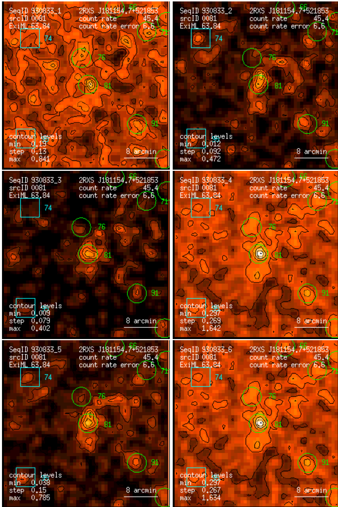
Figure 81: RASS 930833: detection 0081: band rate images, Gaussian filter: (1) PSPC channels 11 – 41, (2) 52 – 90, (3) 91 – 201, (4) 11 – 235, (5) 52 – 201, (6) 11 – 201. Broad band rates in counts/ks. Band rate contour levels in counts/ks/arcmin 2 .
