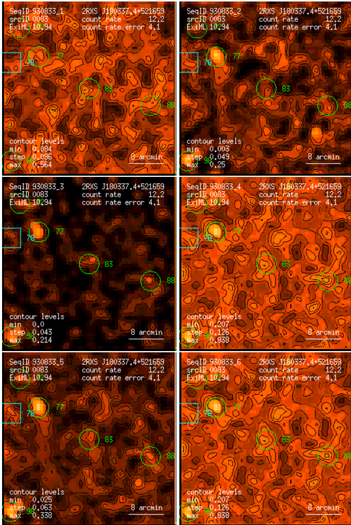
Figure 83: RASS 930833: detection 0083: band rate images, Gaussian filter: (1) PSPC channels 11 – 41, (2) 52 – 90, (3) 91 – 201, (4) 11 – 235, (5) 52 – 201, (6) 11 – 201. Broad band rates in counts/ks. Band rate contour levels in counts/ks/arcmin 2 .
