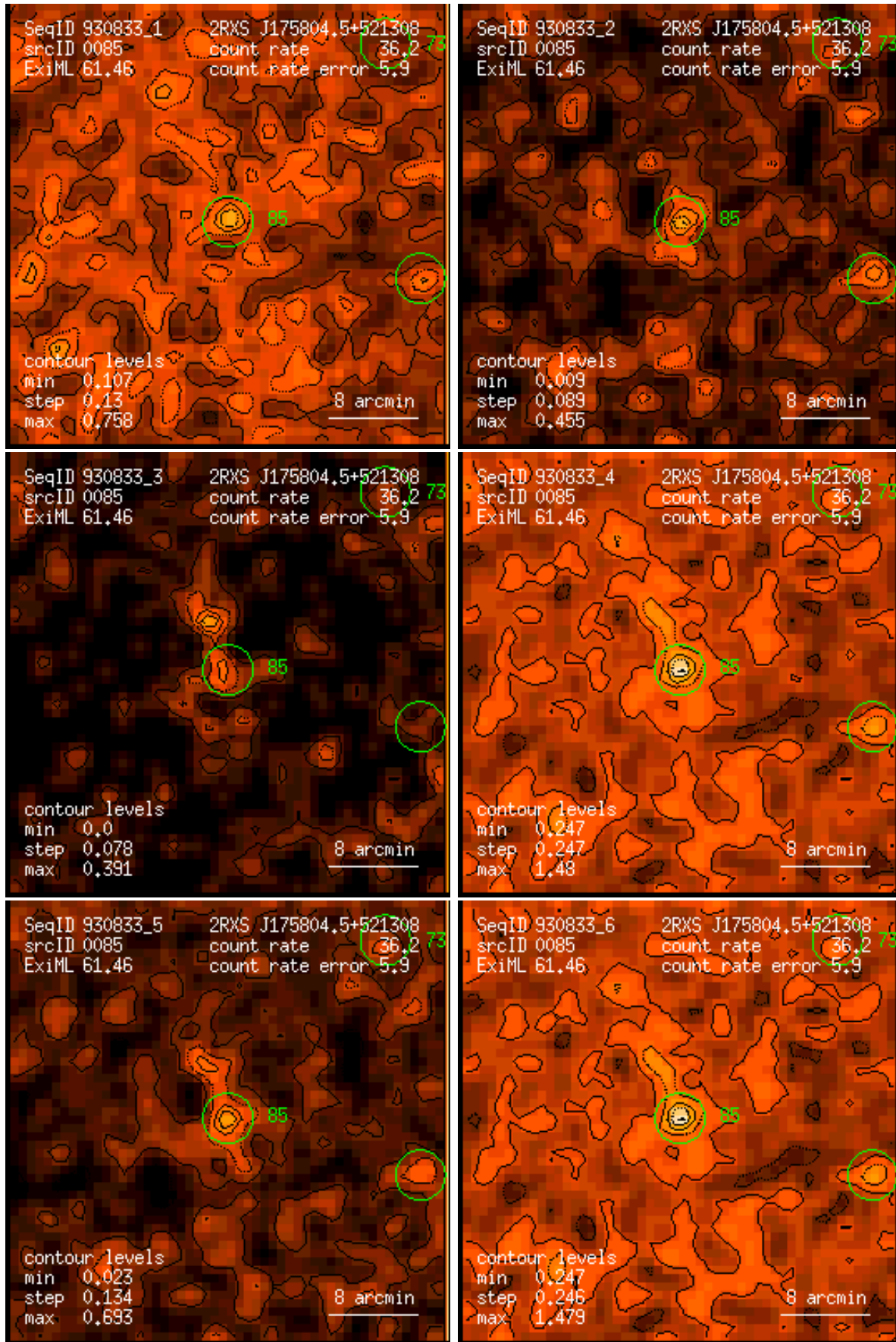
Figure 85: RASS 930833: detection 0085: band rate images, Gaussian filter: (1) PSPC channels 11 – 41, (2) 52 – 90, (3) 91 – 201, (4) 11 – 235, (5) 52 – 201, (6) 11 – 201. Broad band rates in counts/ks. Band rate contour levels in counts/ks/arcmin 2 .
