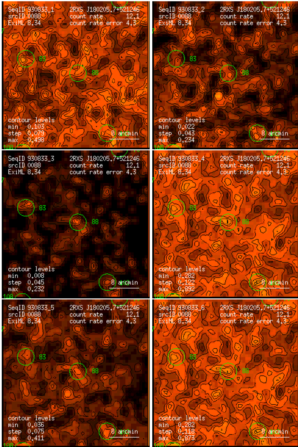
Figure 88: RASS 930833: detection 0088: band rate images, Gaussian filter: (1) PSPC channels 11 – 41, (2) 52 – 90, (3) 91 – 201, (4) 11 – 235, (5) 52 – 201, (6) 11 – 201. Broad band rates in counts/ks. Band rate contour levels in counts/ks/arcmin 2 .
