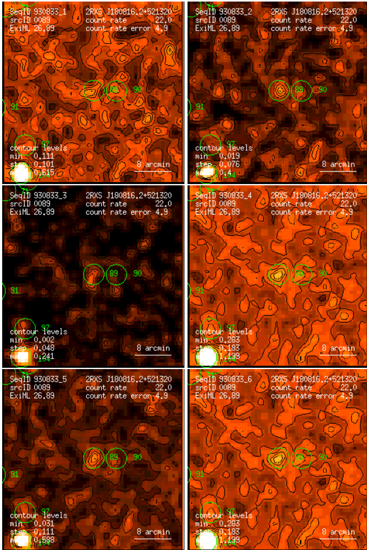
Figure 89: RASS 930833: detection 0089: band rate images, Gaussian filter: (1) PSPC channels 11 – 41, (2) 52 – 90, (3) 91 – 201, (4) 11 – 235, (5) 52 – 201, (6) 11 – 201. Broad band rates in counts/ks. Band rate contour levels in counts/ks/arcmin 2 .
